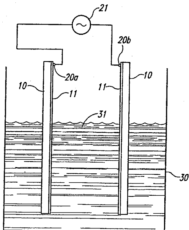
Fig. 2 (Prior Art)
