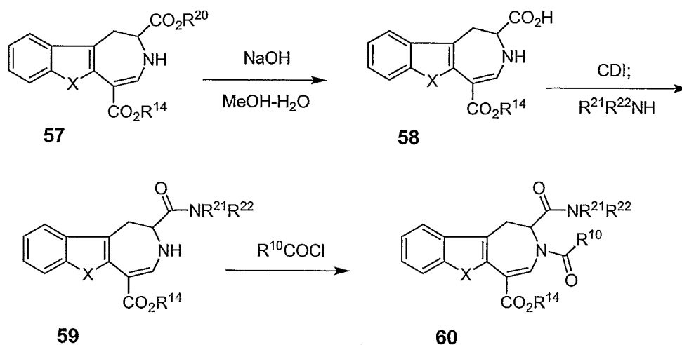
SCHEME 21
