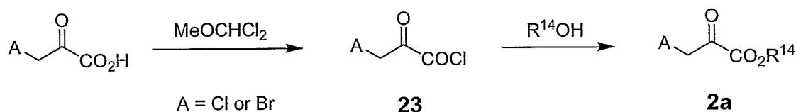
SCHEME 8
