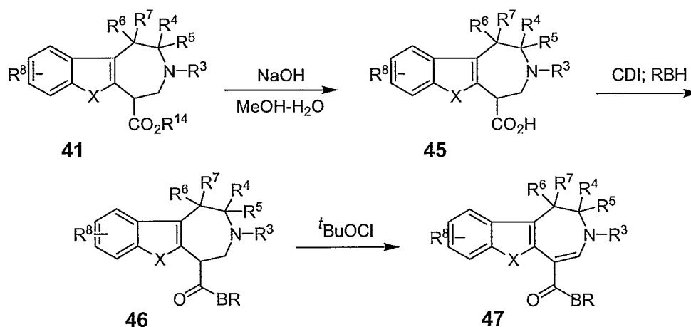
SCHEME 16
