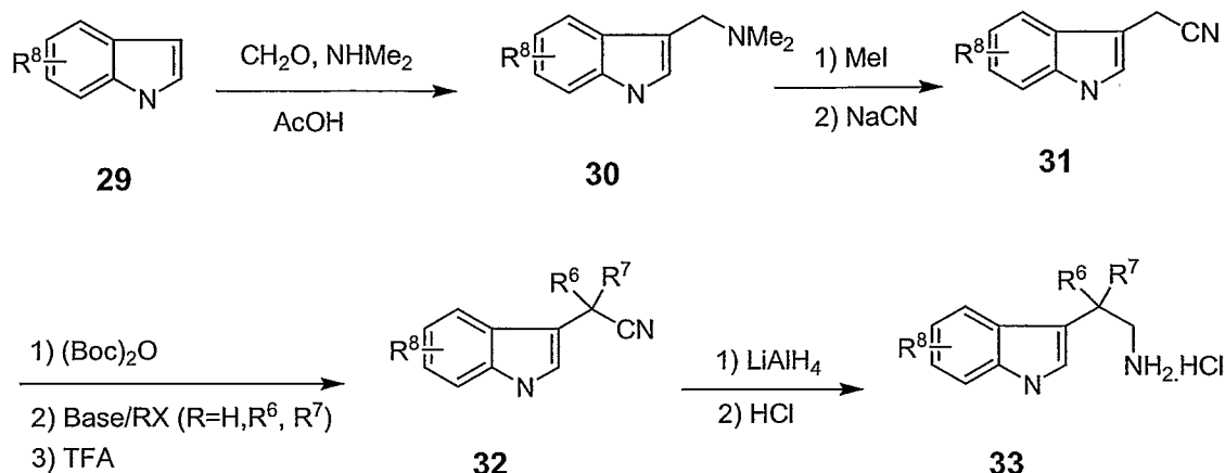
SCHEME 11
