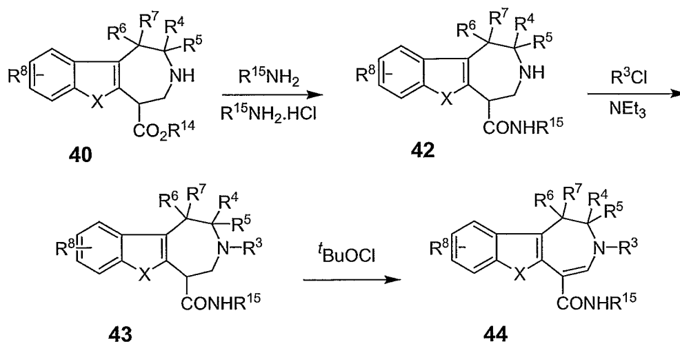
SCHEME 15
