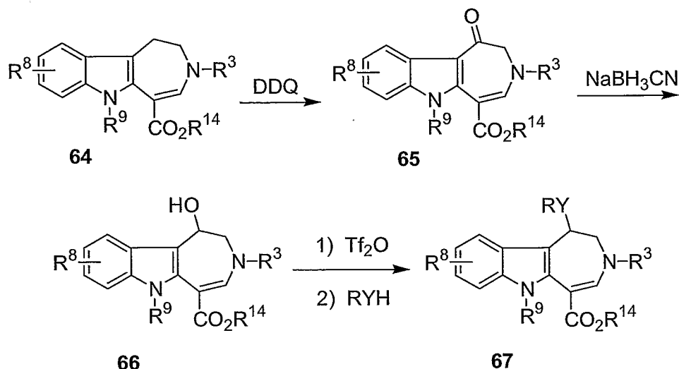
SCHEME 23
