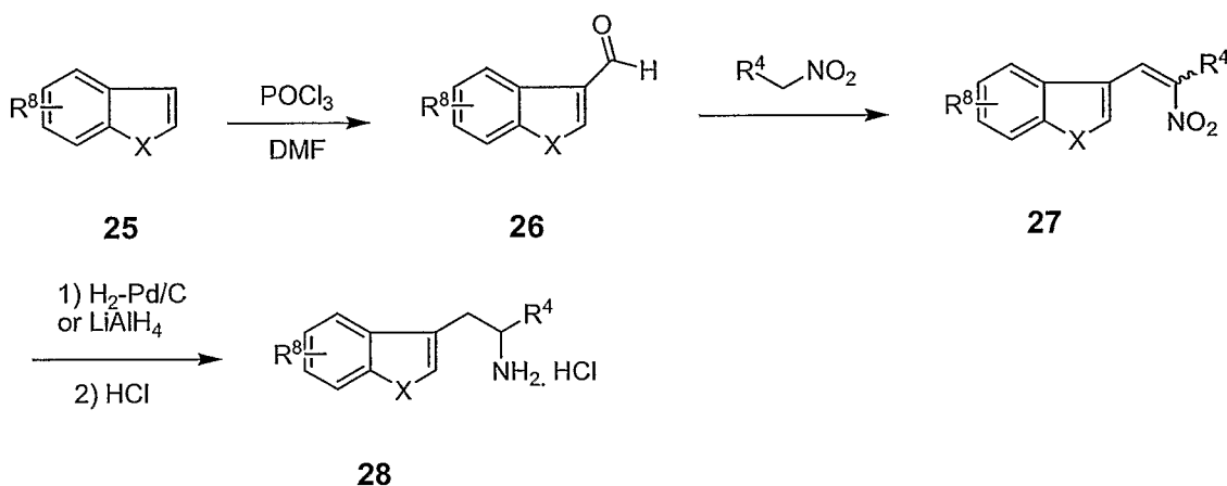
SCHEME 10
