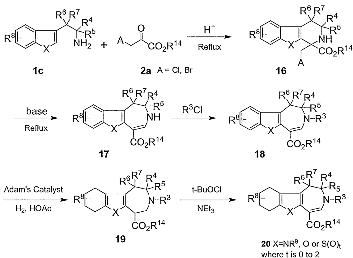
Scheme 6
