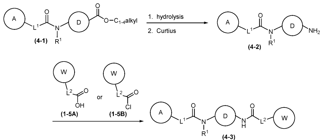
Scheme 4: Representative scheme for synthesis of exemplary compounds of the invention.
