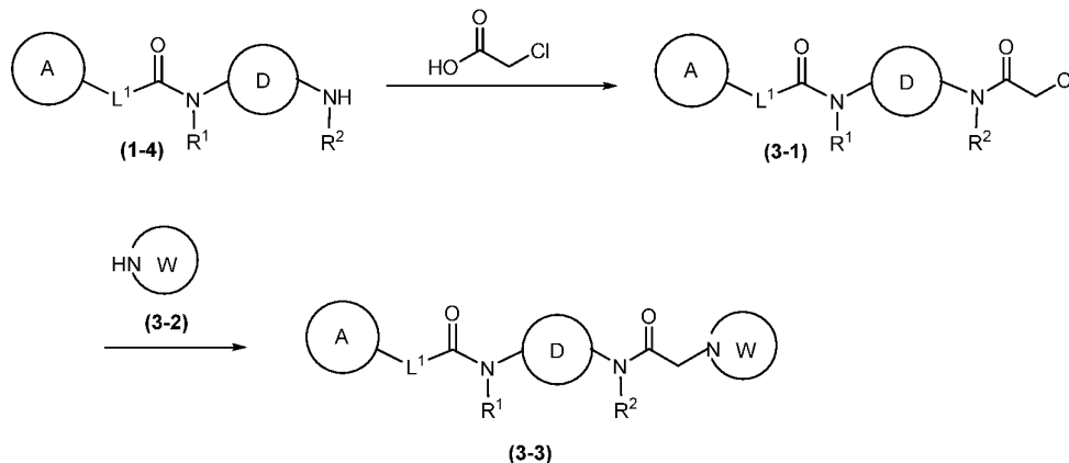
Scheme 3: Representative scheme for synthesis of exemplary compounds of the invention.
