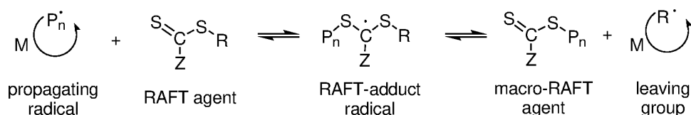
Scheme 1: Proposed mechanism for RAFT polymerisation.
