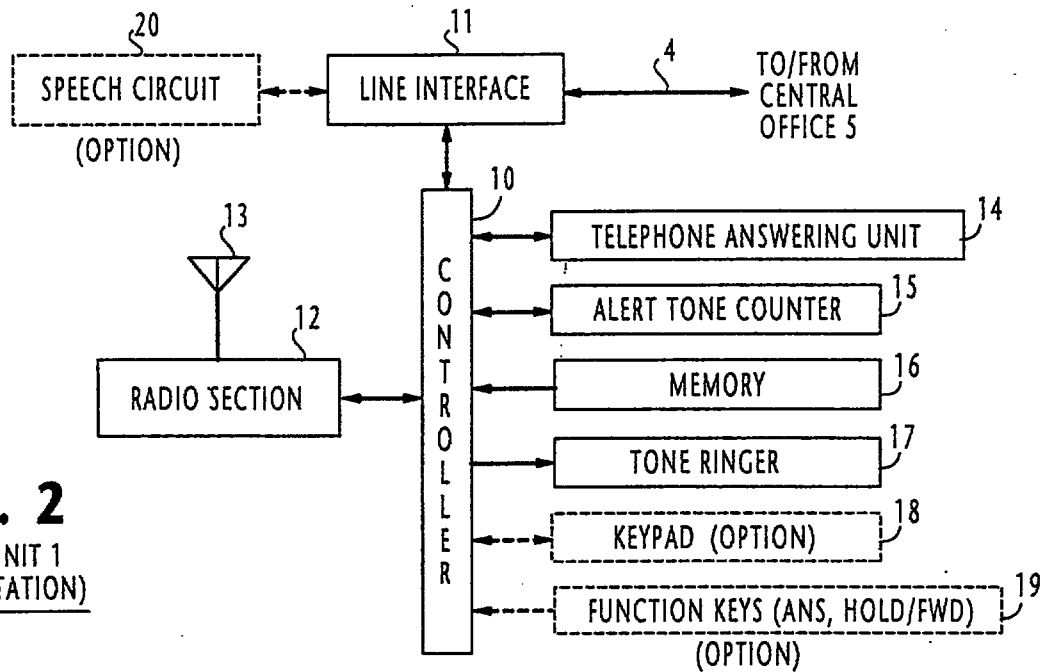
FIG. 3 CORDLESS STATION 2
