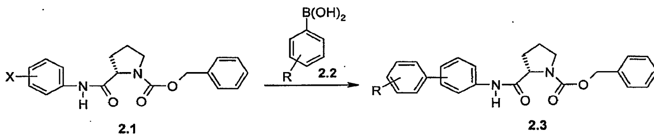
Scheme 2
