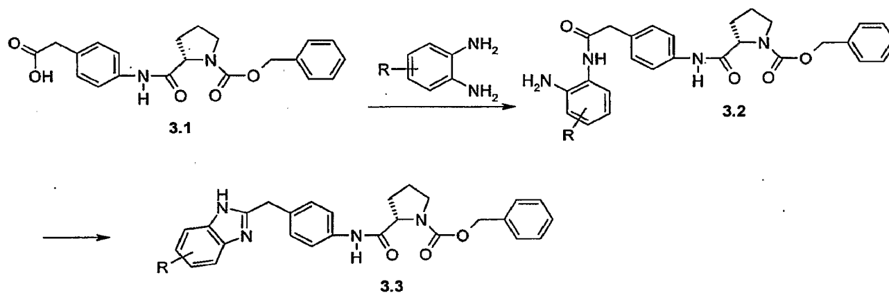
Scheme 3
