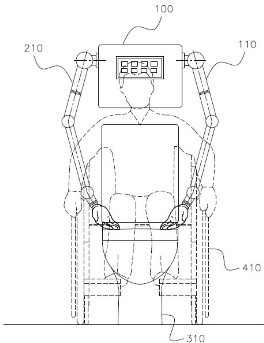
FIGURE 5 — GENERAL ARRANGEMENT OF ROBOTIC ARM IN TOILET FRONT VIEW
