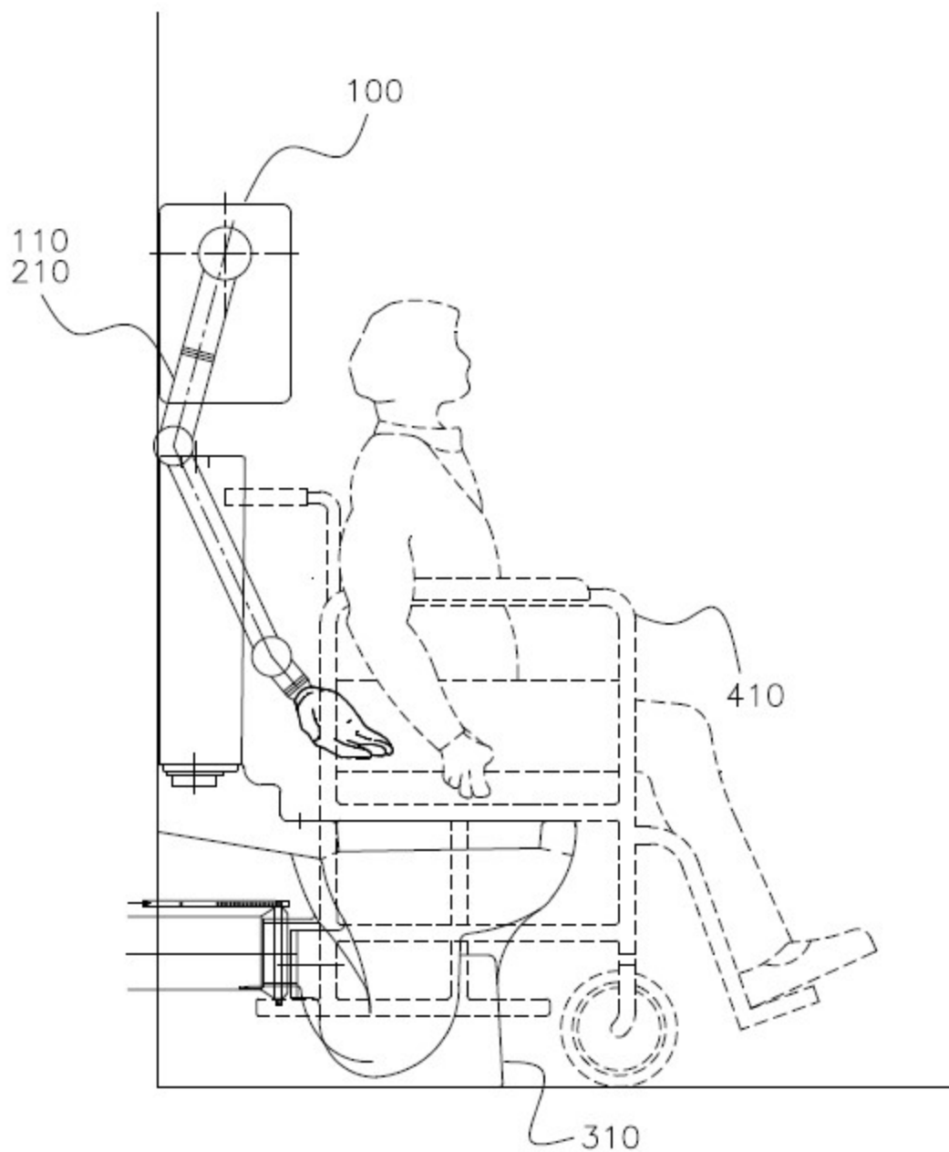
FIGURE 6 – GENERAL ARRANGEMENT OF ROBOTIC ARM IN TOILET SIDE VIEW
