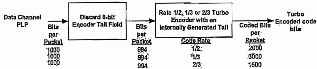
Figure 5.2.1.2.9.6.1.1-1 Data Channel Encoder
