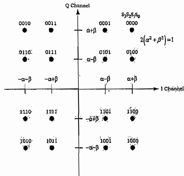
Figure 5.2.1.2.9.6.1.6.3-1 Signal Constellation for Layered Modulation
