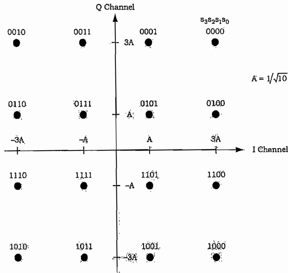
Figure 5.2.1.2.9.6.1.6.2-1 Signal Constellation for 16-QAM Modulation.
