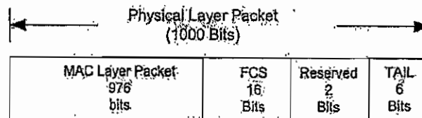
Figure 5.1.2-1 Physical Layer Packet Format
