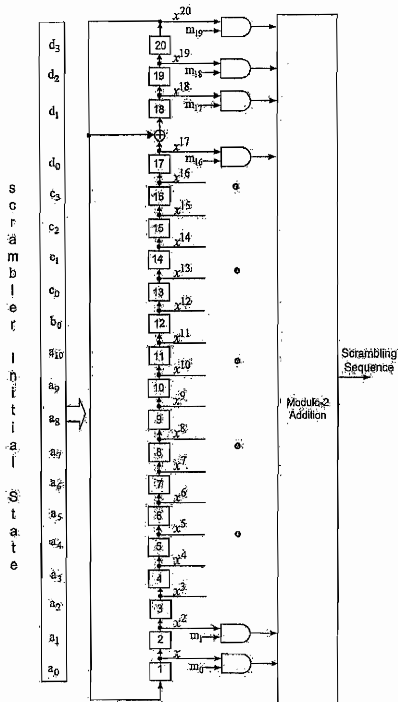
Figure 5.2.1.2.9.1.2.3-1 Slot Bit Scrambler
