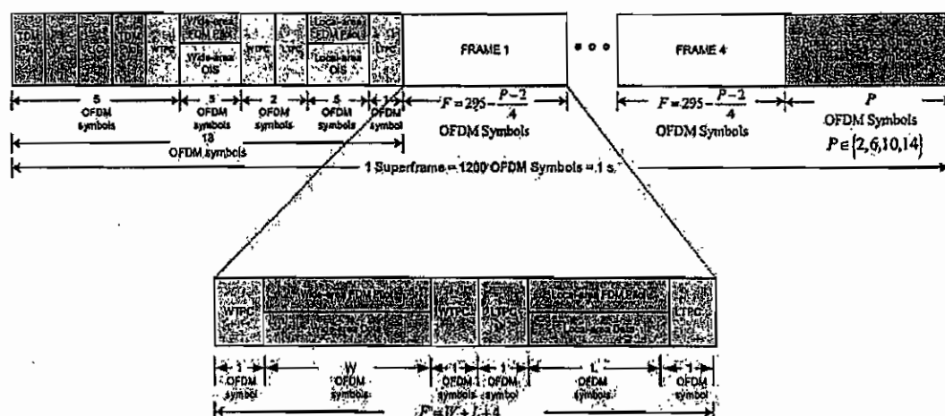
Figure 5.2.1.2.3-2 FLO SuperFrame and Channel Structure
