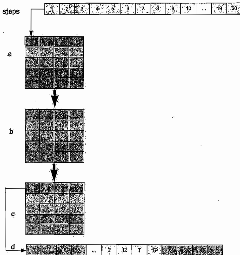
Figure 5.2.1.2.9.2.2-1 Bit Interleaver Operation Example for N = 20
