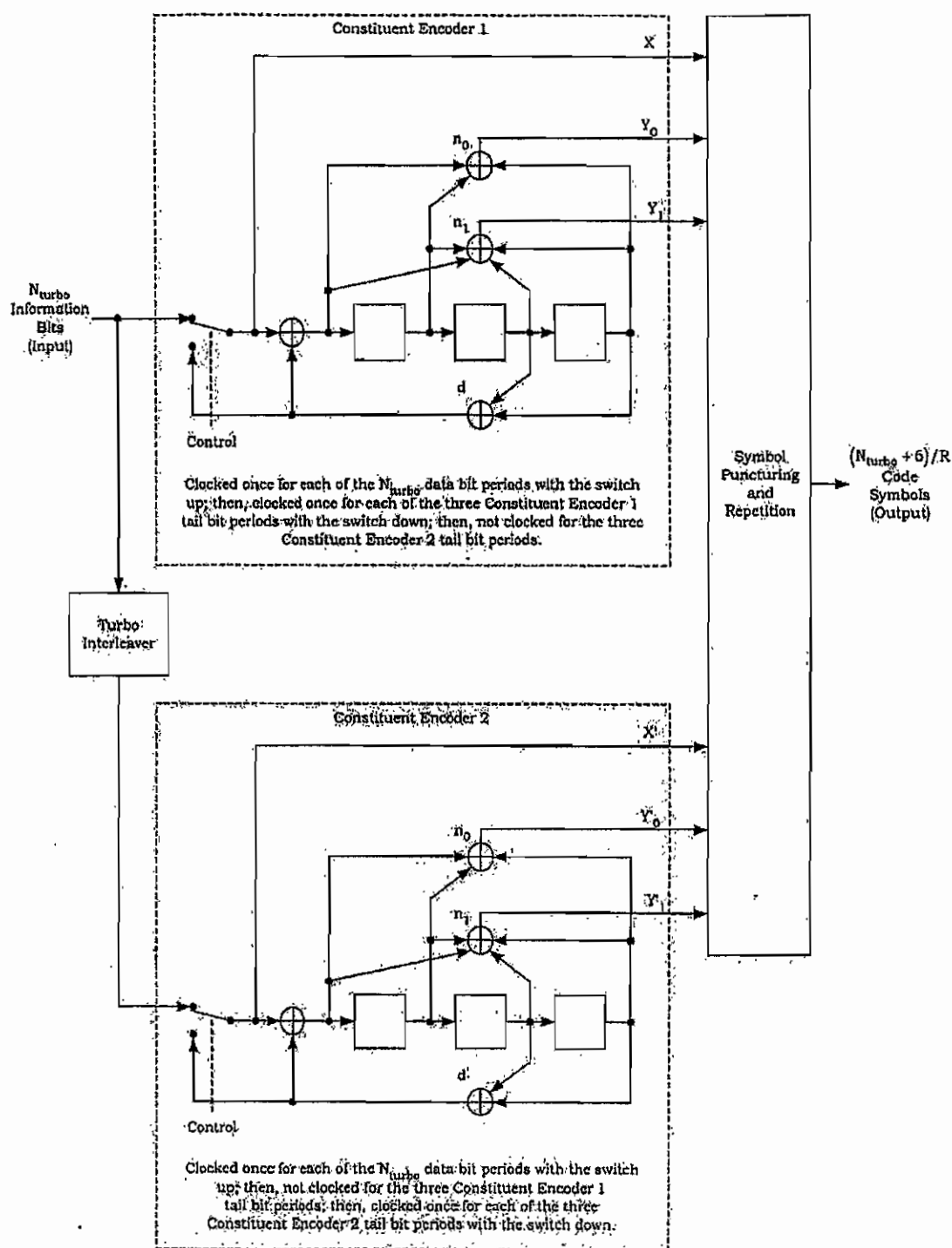
Figure 5.2.1.2.9.2.1.1-1 Turbo Encoder.
