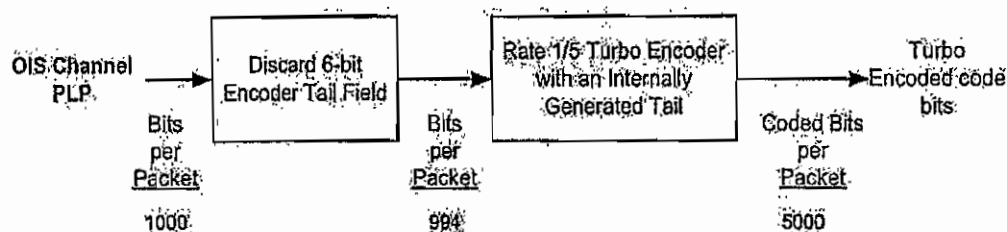
Figure 5.2.1.2.9.2.1-1 Wide-area/Local-area OIS Channel Encoder
