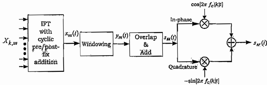
Figure 5.2.1.2.11-1 OFDM Common Operation
