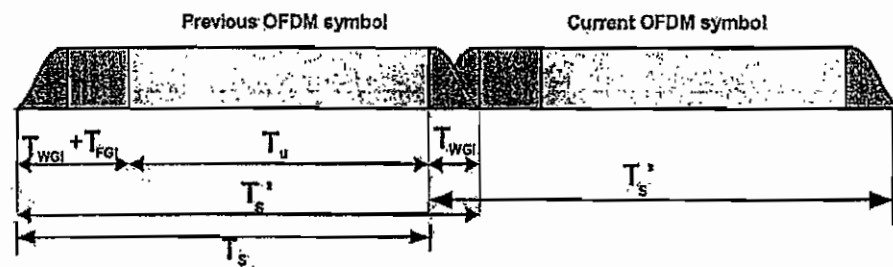
Figure 5.2.1.2.11.3-1 Overlap of Windowed OFDM Symbols
