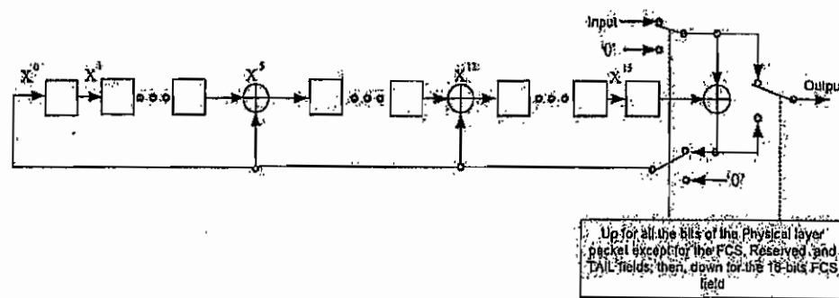
Figure 5.1.4-1 FCS Computation for the Physical Layer Packet
