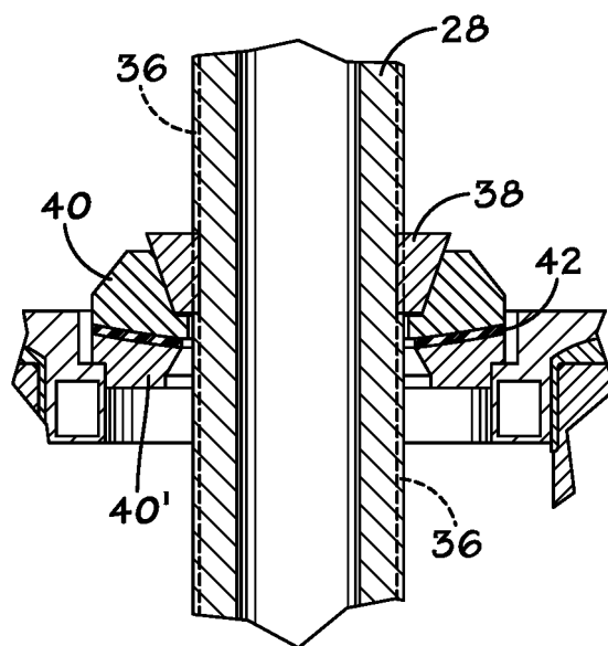
DETAIL B
