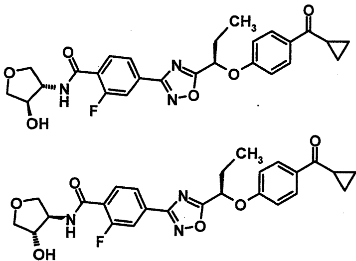
[Chemical Formula 17]
