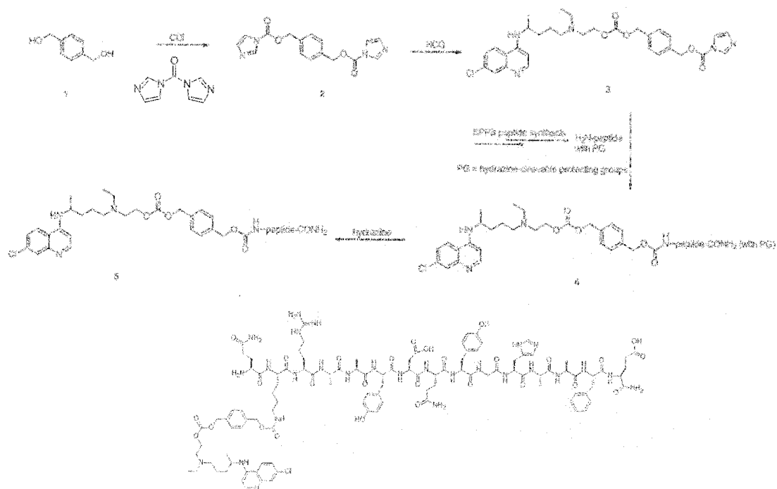
Compound VI
