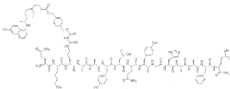
Compound VIII
