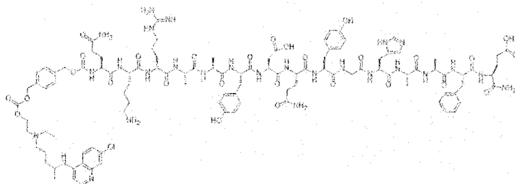
Compound VII
