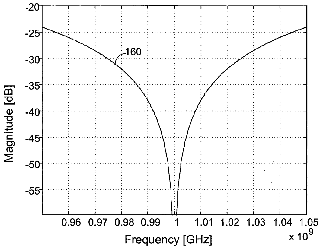
Fig. 4 (Prior Art)
