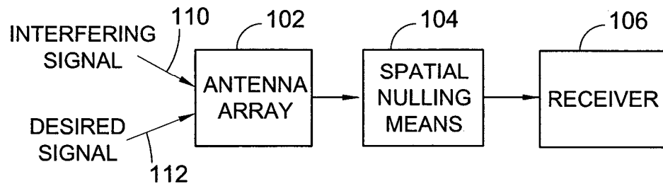
Fig. 1 (Prior Art)
