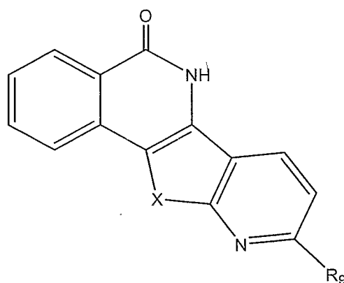
(IV')
