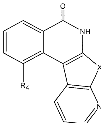
(VIIa')
