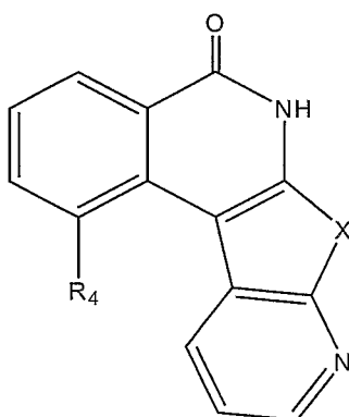
(VIIa')
