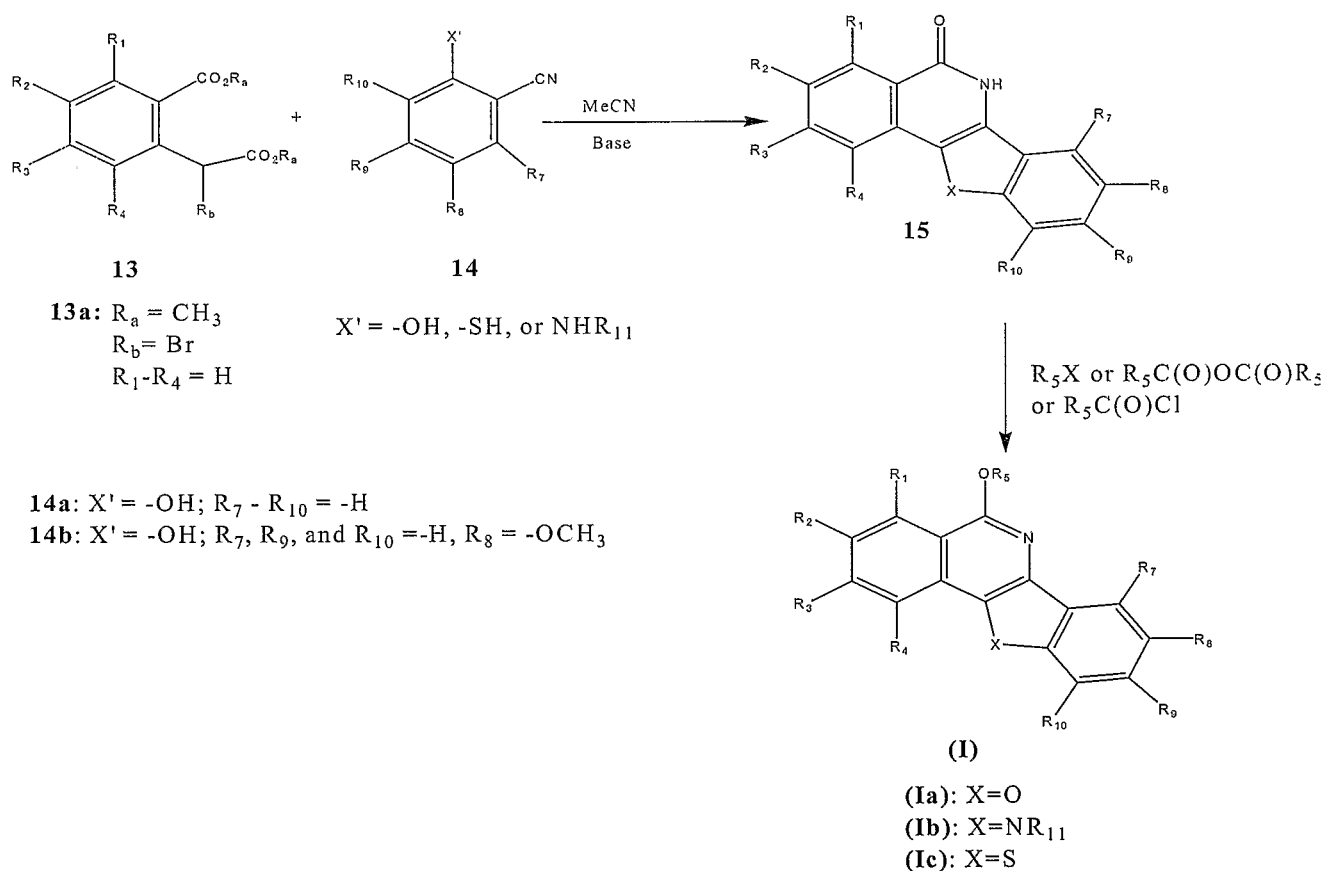
Scheme 2
