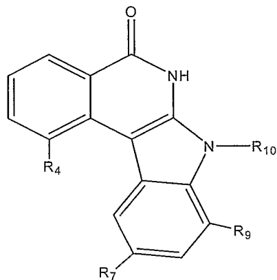
(VI')
