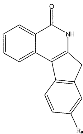
(IIa')
