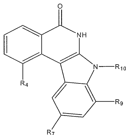
(VI')
