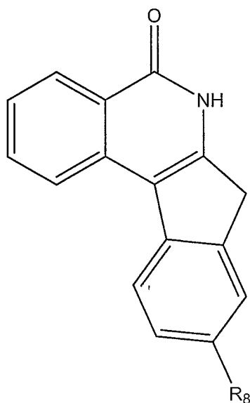
(IIa')
