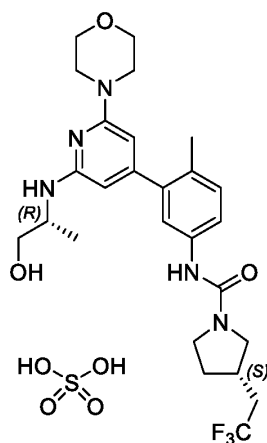
Compound 6
