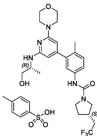
Compound 4
