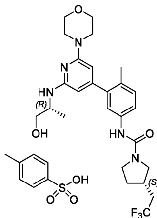
Compound 4
