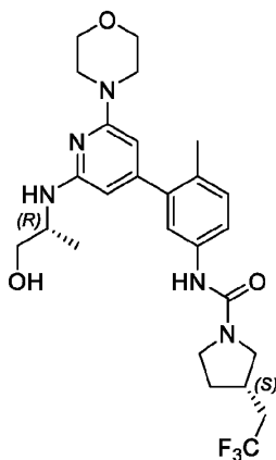
Compound 1
