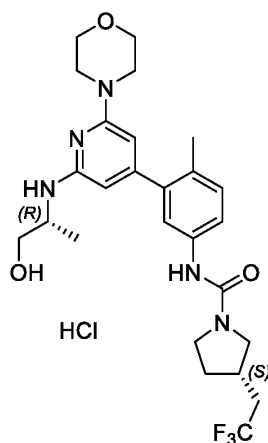
Compound 2
