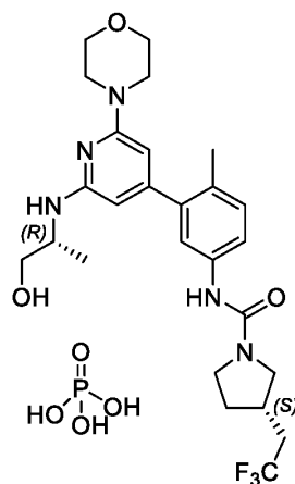
Compound 5
