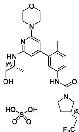
Compound 6
