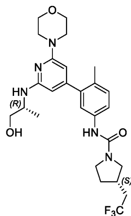
Compound 1
