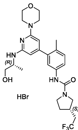
Compound 3
