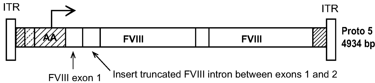
Schematic of Proto 5
