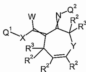
Formula 4.G.2
