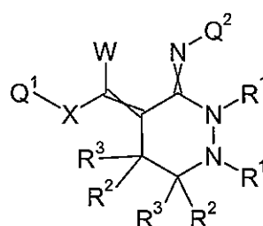
Formula 8.D.8
