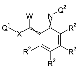
Formula 1.C.5
