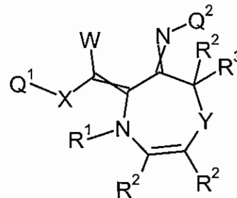
Formula 6.L.3
