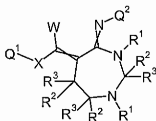
Formula 8.E.8
