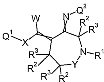
Formula 6.D.5
