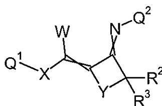
Formula 4.K.1
