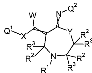
Formula 7.E.3
