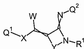
Formula 8.G.1
