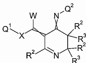
Formula 5.E.4
