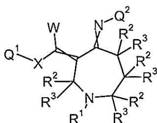
Formula 5.I.1
