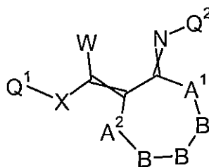
Formula I-d
