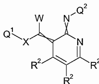
Formula 5.M.4
