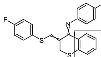
Example 1-35
