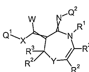
Formula 8.E.2
