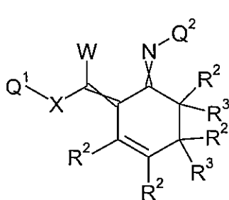
Formula 1.C.4
