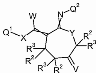
Formula 3.E.2
