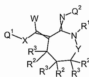
Formula 8.E.6
