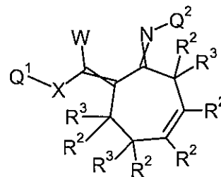
Formula 1.D.3
