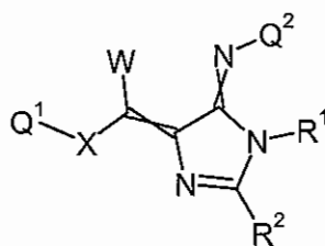
Formula 8.L.2
