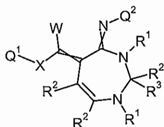
Formula 8.E.13
