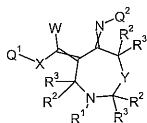
Formula 6.D.3
