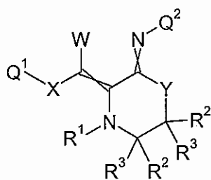
Formula 7.M.1
