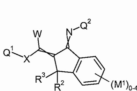
Formula 1.B.5
