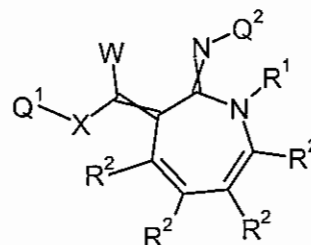
Formula 5.N.5
