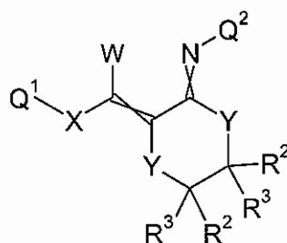
Formula 7.H.1
