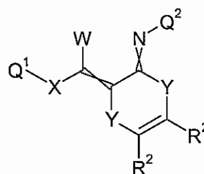
Formula 7.H.2
