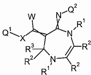
Formula 8.E.4
