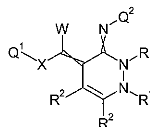
Formula 8.D.9
