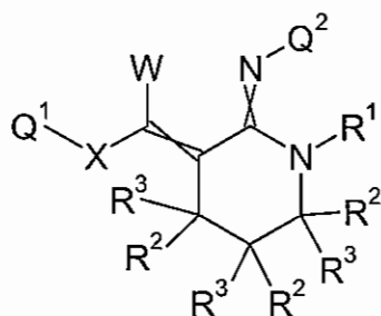
Formula 5.M.1
