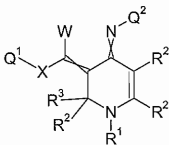
Formula 5.E.2
