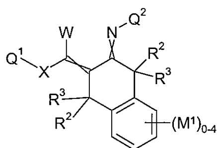
Formula 1.C.7
