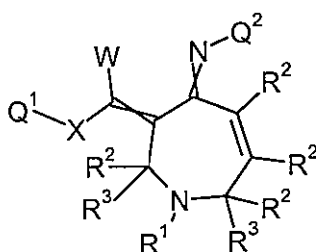
Formula 5.I.2
