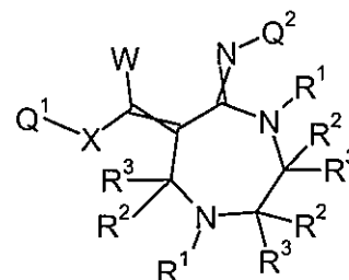
Formula 8.E.3
