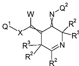
Formula 5.D.4
