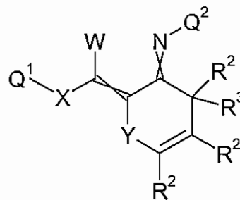
Formula 4.M.3
