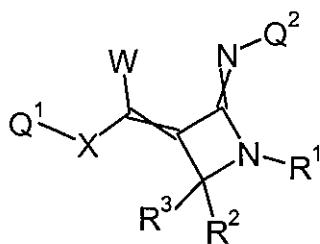
Formula 5.K.1
