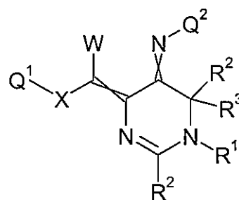
Formula 6.K.3
