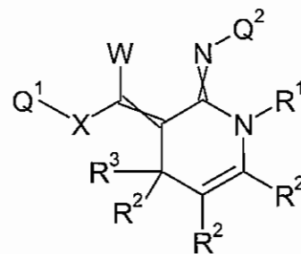
Formula 5.M.3
