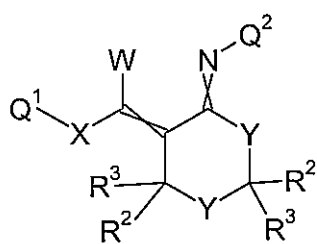
Formula 7.D.1
