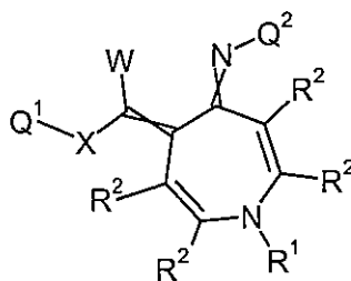
Formula 5.H.4
