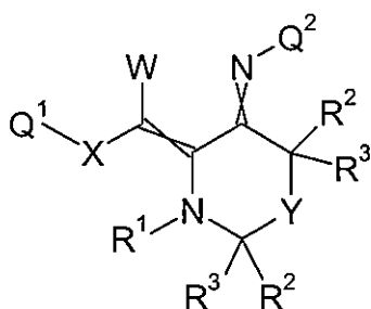
Formula 6.K.4
