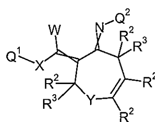
Formula 4.I.3
