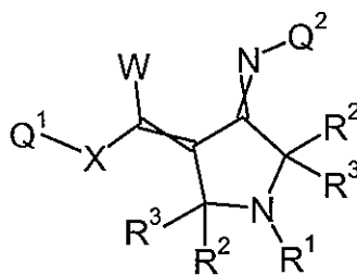
Formula 5.B.1
