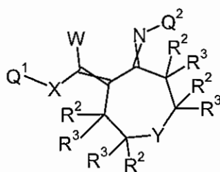
Formula 4.H.1
