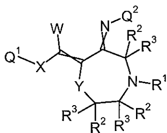
Formula 6.H.4
