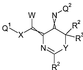
Formula 6.K.5
