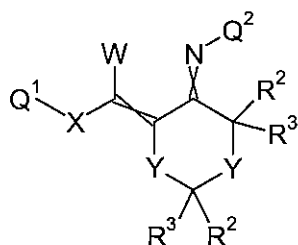
Formula 6.G.1
