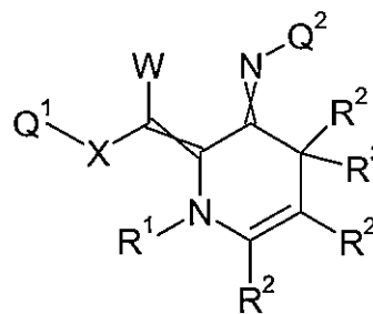
Formula 5.R.3
