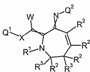
Formula 5.S.4
