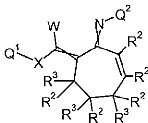
Formula 1.D.2
