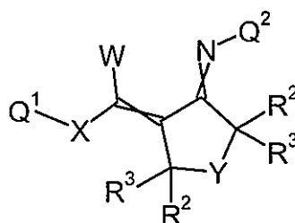
Formula 4.B.1
