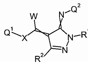
Formula 8.C.3
