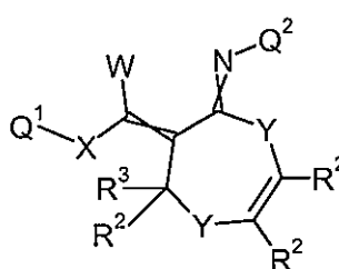
Formula 7.E.2
