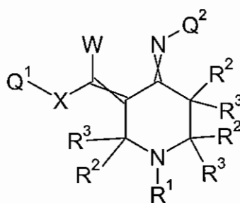
Formula 5.E.1
