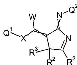
Formula 5.L.3
