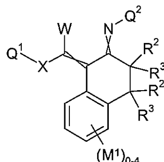
Formula 1.C.8
