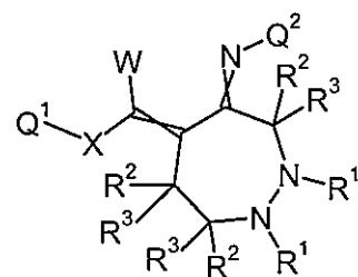
Formula 6.D.3
