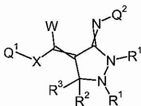
Formula 8.C.2
