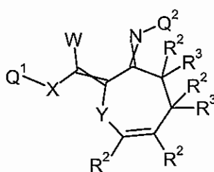
Formula 4.N.2
