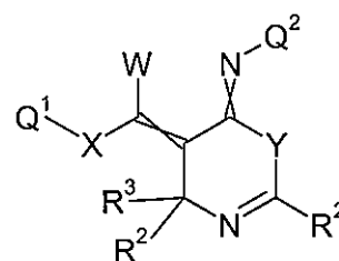
Formula 7.D.6
