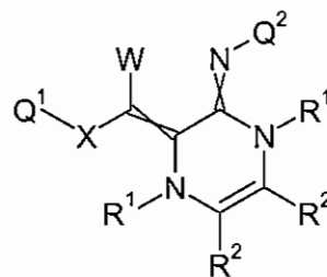
Formula 8.M.2
