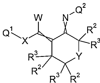
Formula 4.D.1
