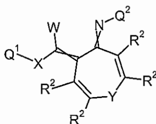
Formula 4.H.4
