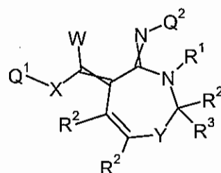
Formula 8.E.14
