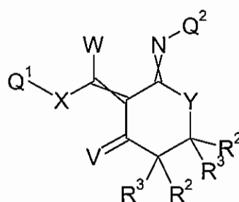
Formula 3.C.3
