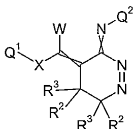
Formula 8.D.1
