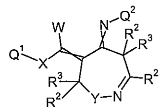
Formula 6.D.12
