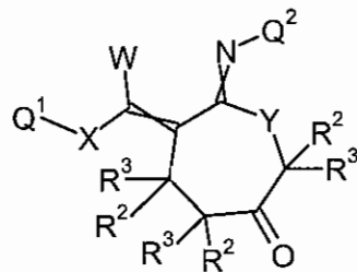
Formula 3.F.2
