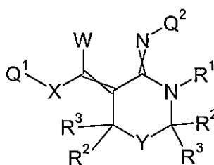
Formula 8.D.5
