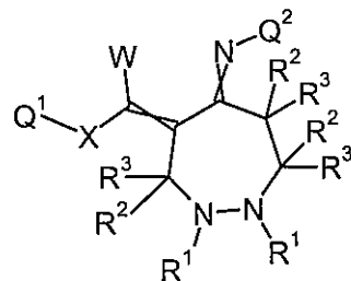
Formula 6.D.11
