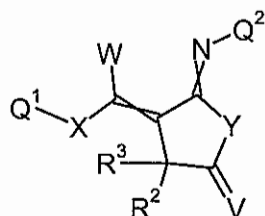
Formula 3.A.1
