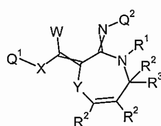
Formula 8.J.3
