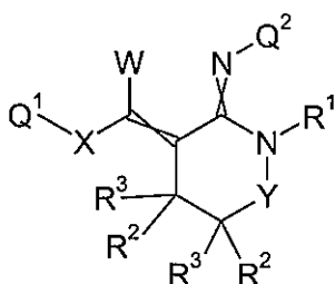
Formula 8.D.7
