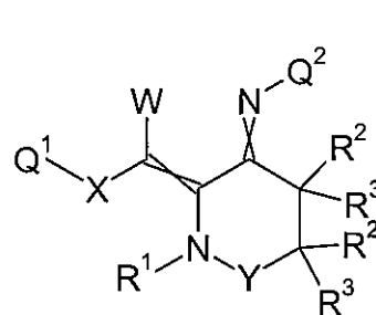
Formula 6.K.6
