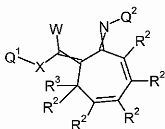
Formula 1.D.7
