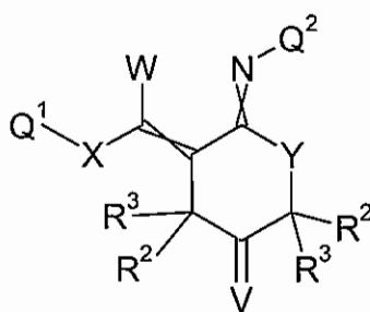
Formula 3.C.2
