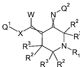
Formula 5.D.1
