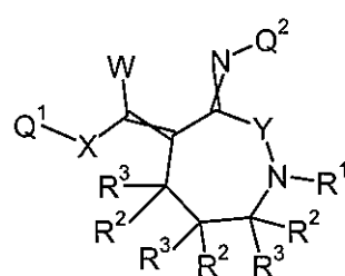
Formula 7.E.9
