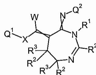
Formula 8.E.9
