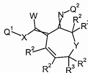
Formula 4.G.3
