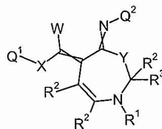
Formula 7.E.12
