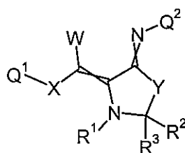
Formula 7.L.1
