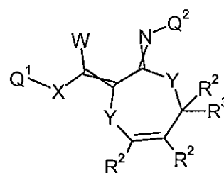
Formula 7.I.3
