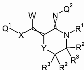
Formula 8.I.1
