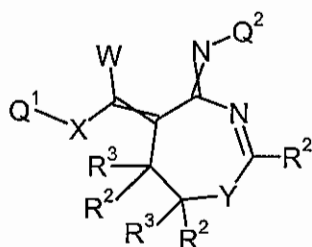
Formula 8.E.7
