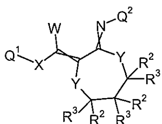
Formula 7.I.1
