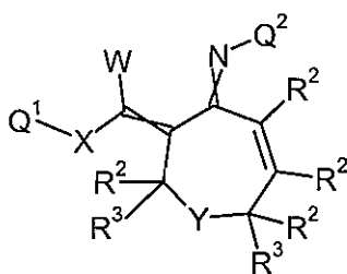
Formula 4.I.2
