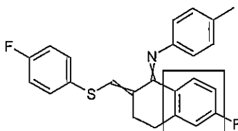
Example 1-16
