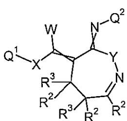
Formula 7.E.8
