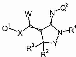
Formula 8.C.1
