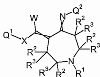
Formula 5.H.1
