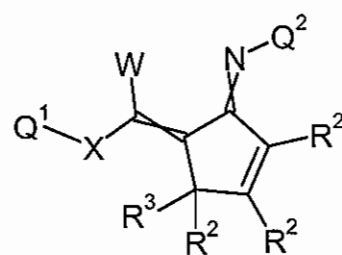
Formula 1.B.3
