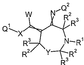
Formula 6.D.2
