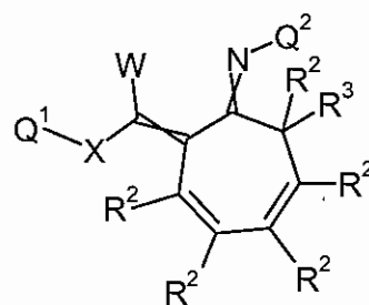
Formula 1.D.6
