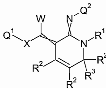
Formula 5.M.2
