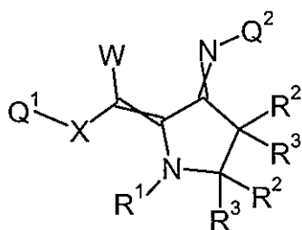
Formula 5.Q.1
