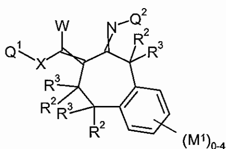
Formula 1.D.10
