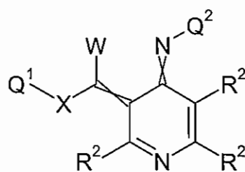
Formula 5.E.3
