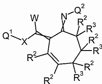
Formula 1.D.5
