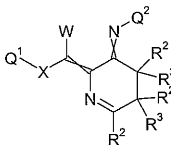
Formula 5.R.5
