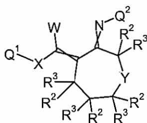
Formula 4.G.1
