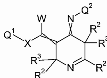
Formula 5.E.5
