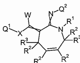
Formula 5.N.2
