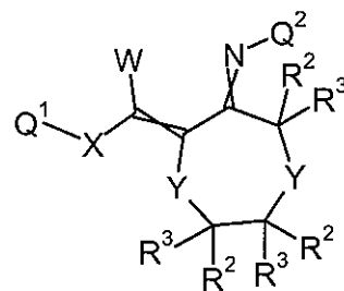
Formula 6.H.6
