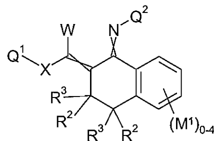
Formula 1.C.6
