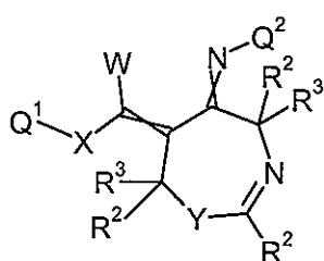
Formula 6.D.4
