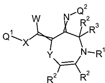
Formula 6.H.5
