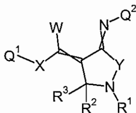
Formula 7.C.1
