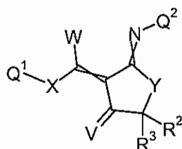
Formula 3.A.2
