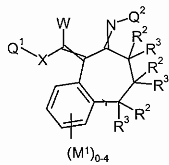
Formula 1.D.12
