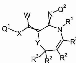
Formula 8.J.2
