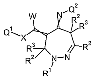
Formula 6.D.13
