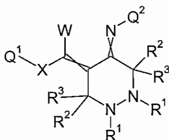
Formula 6.C.1
