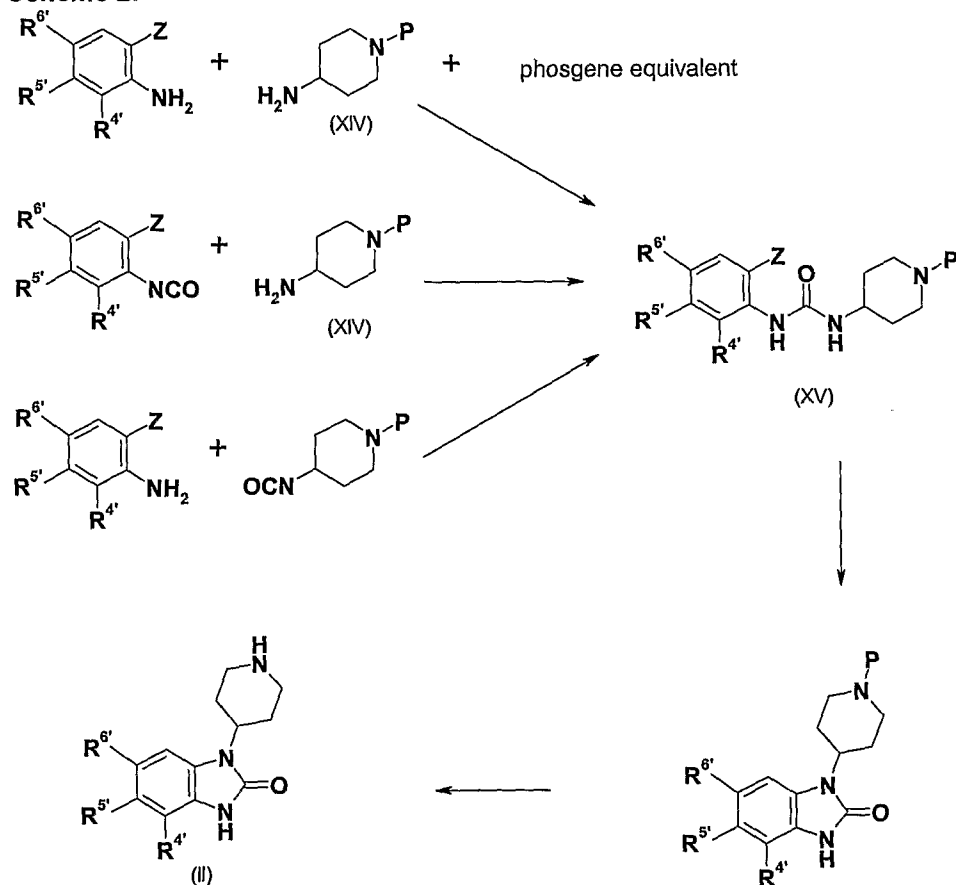
Scheme 2.
