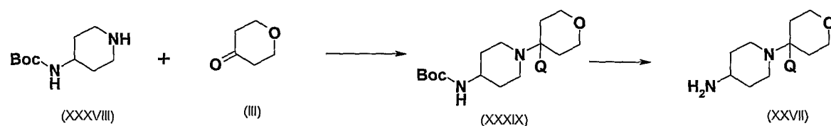
Scheme 15.
