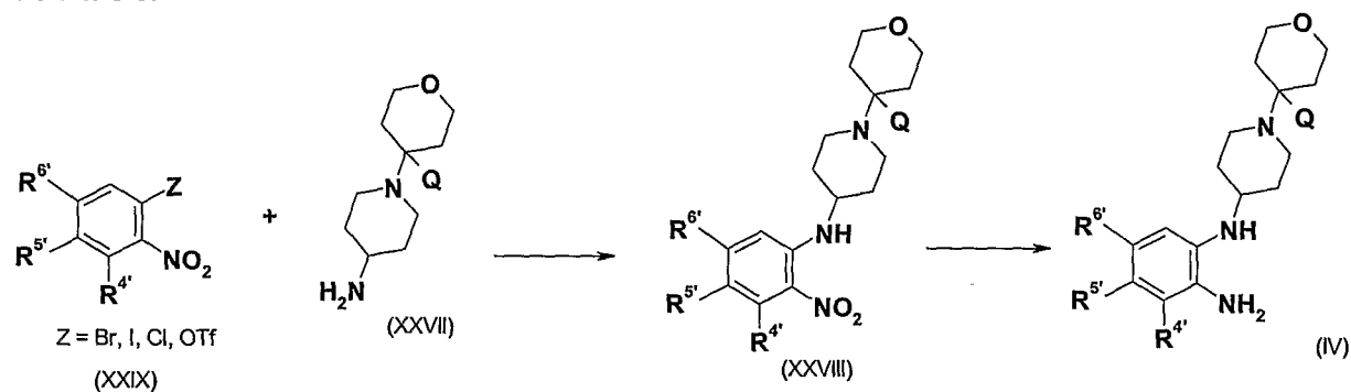
Scheme 9.
