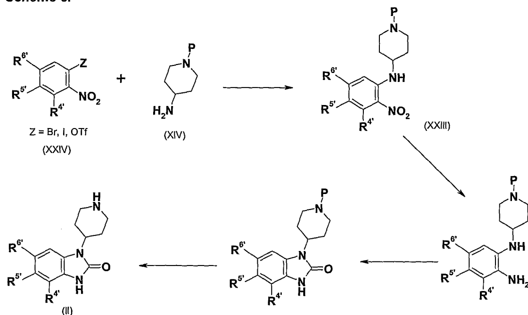
Scheme 6.
