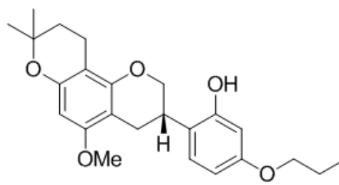
<Compound 12b>
