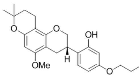
<Compound 12b>
