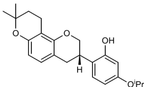
<Compound 3b>
