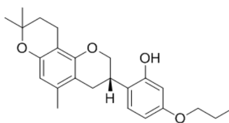
<Compound 10b>
