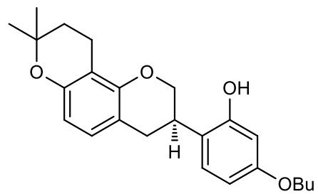
<Compound 4a>
