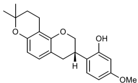
<Compound 13b>.
