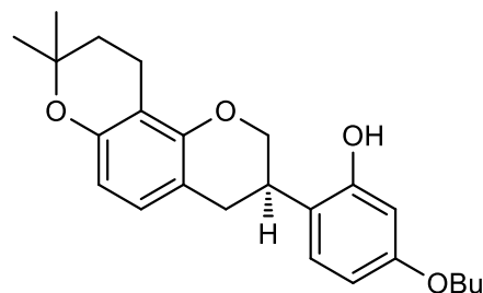
<Compound 4a>
