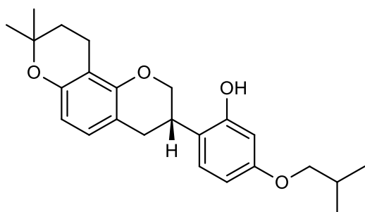
<Compound 5b>
