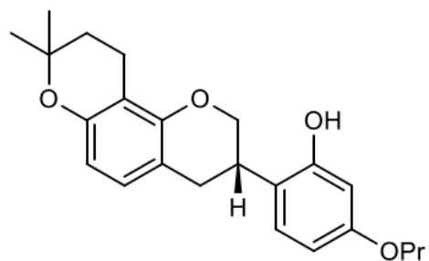
<Compound 2b>
