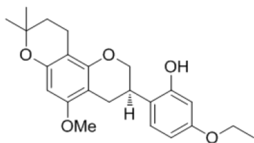
<Compound 11a>
