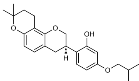
<Compound 5a>
