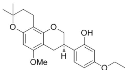
<Compound 11a>
