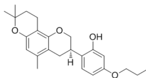
<Compound 10a>
