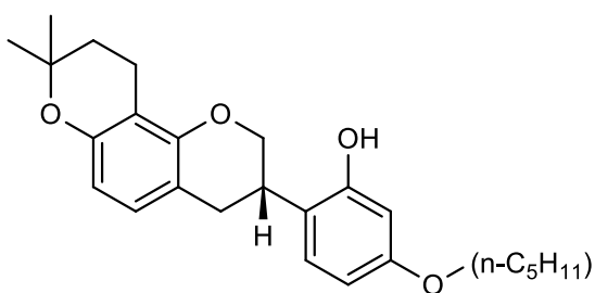
<Compound 6b>
