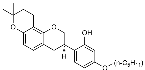
<Compound 6a>
