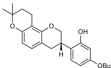
<Compound 4b>
