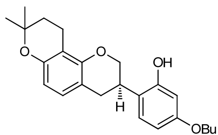
<Compound 4a>
