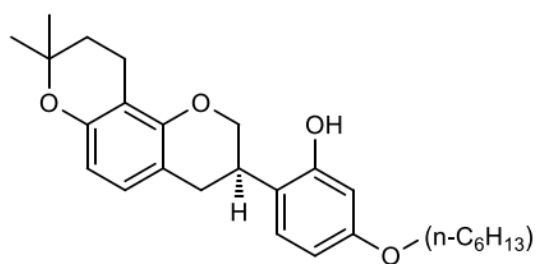
<Compound 7a>
