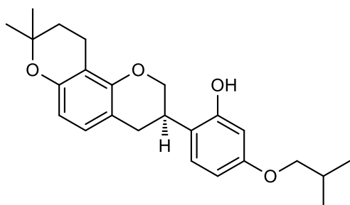
<Compound 5a>
