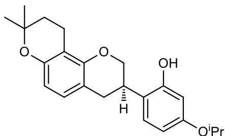
<Compound 3a>
