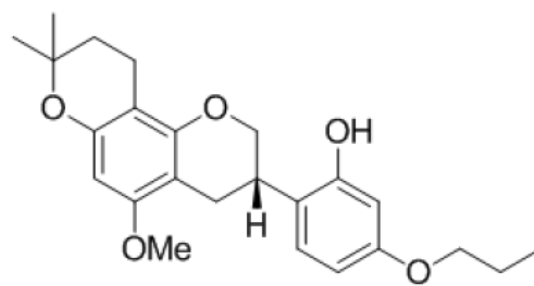
<Compound 12b>
