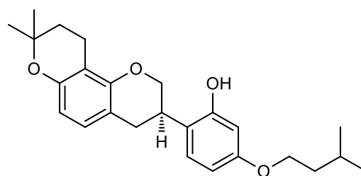
<Compound 8a>
