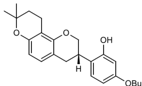
<Compound 4b>
