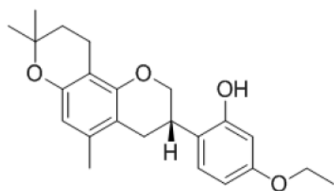
<Compound 9b>
