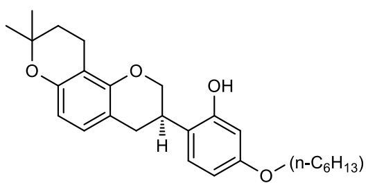
<Compound 1a>
