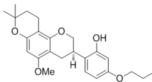
<Compound 12a>
