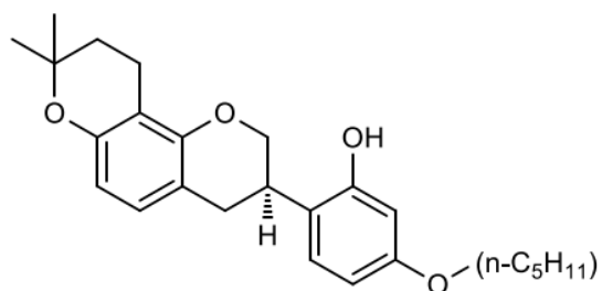
<Compound 6a>
