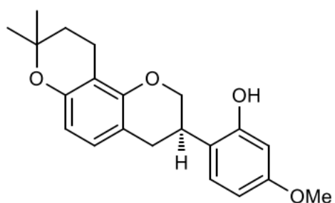
<Compound 13a>.
