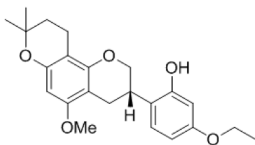
<Compound 11b>
