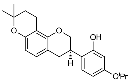
<Compound 3a>
