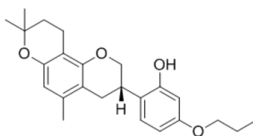
<Compound 10b>
