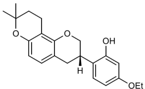
<Compound 1b>
