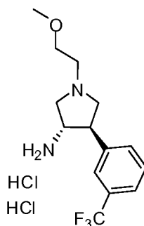
(3S,4R)-1-(2-methoxyethyl)-4-(3-(trifluoromethyl)phenyl)pyrrolidin-3-amine dihydrochloride
