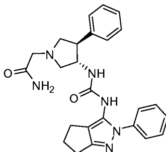
2-(((3R,4S)-3-phenyl-4-(3-(2-phenyl-2,4,5,6-tetrahydrocyclopenta[c]pyrazol-3-yl)ureido)pyrrolidin-1-yl)acetamide
