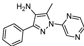
5-methyl-3-phenyl-1-(pyrazin-2-yl)-1H-pyrazol-4-amine
