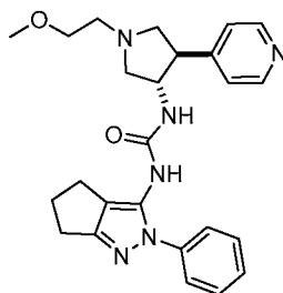
1-( trans -1-(2-methoxyethyl)-4-(pyridin-4-yl)pyrrolidin-3-yl)-3-(2-phenyl-2,4,5,6-tetrahydrocyclopenta[ c ]pyrazol-3-yl)urea
