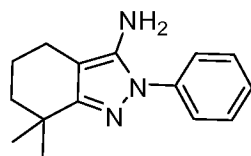
7,7-dimethyl-2-phenyl-4,5,6,7-tetrahydro-2H-indazol-3-amine
