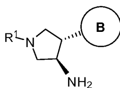
enantiomer 2 of II-A
