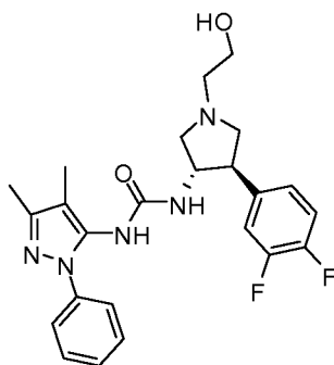
1-(((3S,4R)-4-(3,4-difluorophenyl)-1-(2-hydroxyethyl)pyrrolidin-3-yl)-3-(3,4-dimethyl-1-phenyl-1H-pyrazol-5-yl)urea
