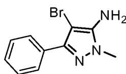
4-bromo-1-methyl-3-phenyl-1H-pyrazol-5-amine
