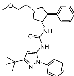
1-(3- tert -butyl-1-phenyl-1 H -pyrazol-5-yl)-3-( trans -1-(2-methoxyethyl)-4-phenylpyrrolidin-3-yl)urea
