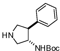
tert-butyl trans-4-phenylpyrrolidin-3-ylcarbamate
