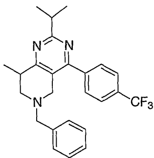
Example 96; 6-Benzyl-2-isopropyl-8-methyl-4-(4-trifluoromethyl-phenyl)-5,6,7,8-tetrahydro-pyrido[4,3-d]pyrimidine.
