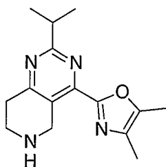
Example 153; 4-(4,5-Dimethyl-oxazol-2-yl)-2-isopropyl-5,6,7,8-tetrahydro-pyrido[4,3-d]pyrimidine.
