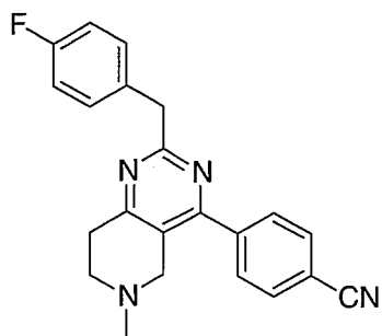
Example 15; 4-[2-(4-Fluoro-benzyl)-6-methyl-5,6,7,8-tetrahydro-pyrido[4,3-d]pyrimidin-4-yl]-benzonitrile.
