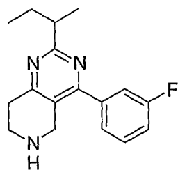
Example 43; 2-sec-Butyl-4-(3-fluoro-phenyl)-5,6,7,8-tetrahydro-pyrido[4,3-d]pyrimidine.
