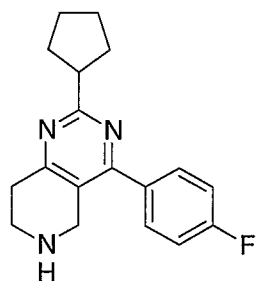
10 Example 17; 2-Cyclopentyl-4-(4-fluoro-phenyl)-5,6,7,8-tetrahydro-pyrido[4,3-d]pyrimidine.
