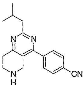
Example 40; 4-(2-Isobutyl-5,6,7,8-tetrahydro-pyrido[4,3-d]pyrimidin-4-yl)-benzonitrile.
