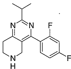
Example 27; 4-(2,4-Difluoro-phenyl)-2-isopropyl-5,6,7,8-tetrahydro-pyrido[4,3-d]pyrimidine.
