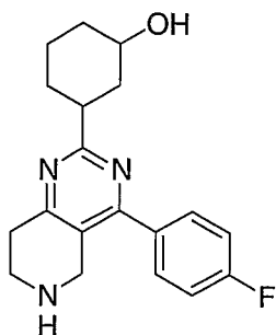
Example 130; 3-[4-(4-Fluoro-phenyl)-5,6,7,8-tetrahydro-pyrido[4,3-d]pyrimidin-2-yl]-cyclohexanol.
