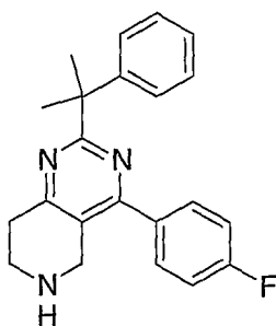
Example 128; 4-(4-Fluoro-phenyl)-2-(1-methyl-1-phenyl-ethyl)-5,6,7,8-tetrahydro-pyrido[4,3-d]pyrimidine.
