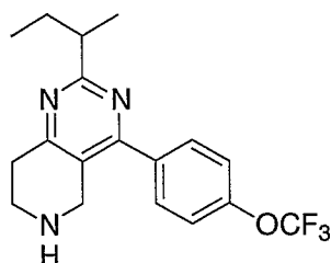
Example 45; 2-sec-Butyl-4-(4-trifluoromethoxy-phenyl)-5,6,7,8-tetrahydro-pyrido[4,3-d]pyrimidine.
