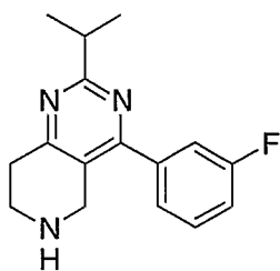
Example 25; 4-(3-Fluoro-phenyl)-2-isopropyl-5,6,7,8-tetrahydro-pyrido[4,3-d]pyrimidine.
