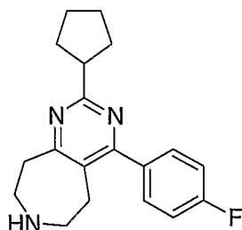
Example 46; 2-Cyclopentyl-4-(4-fluoro-phenyl)-6,7,8,9-tetrahydro-5H-pyrimido[4,5-d]azepine.
