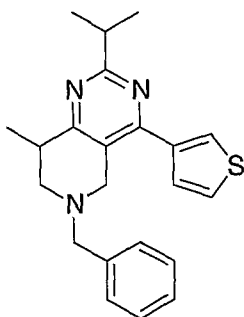
10 Example 98; 6-Benzyl-2-isopropyl-8-methyl-4-thiophen-3-yl-5,6,7,8-tetrahydro-pyrido[4,3-d]pyrimidine.
