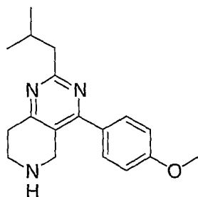
5 Example 41; 2-Isobutyl-4-(4-methoxy-phenyl)-5,6,7,8-tetrahydro-pyrido[4,3-d]pyrimidine.
