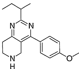
Example 44; 2-sec-Butyl-4-(4-methoxy-phenyl)-5,6,7,8-tetrahydro-pyrido[4,3-d]pyrimidine.
