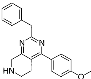
Example 78; 2-Benzyl-4-phenyl-5,6,7,8-tetrahydro-pyrido[3,4-d]pyrimidine.
