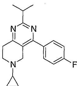
Example 160; 6-Cyclopropyl-4-(4-fluoro-phenyl)-2-isopropyl-5,6,7,8-tetrahydro-pyrido[4,3-d]pyrimidine.
