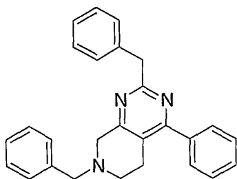
5 Example 72; 2,7-Dibenzyl-4-phenyl-5,6,7,8-tetrahydro-pyrido[3,4-d]pyrimidine.
