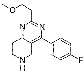
Example 126; 4-(4-Fluoro-phenyl)-2-(2-methoxy-ethyl)-5,6,7,8-tetrahydro-pyrido[4,3-d]pyrimidine.
