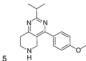
Example 30; 2-Isopropyl-4-(4-methoxy-phenyl)-5,6,7,8-tetrahydro-pyrido[4,3-d]pyrimidine.
