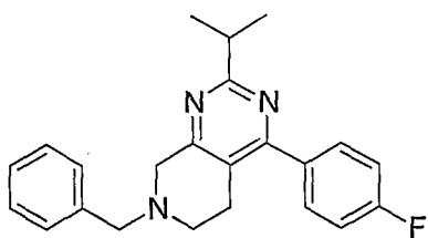
Example 74; 7-Benzyl-4-(4-fluoro-phenyl)-2-isopropyl-5,6,7,8-tetrahydro-pyrido[3,4-d]pyrimidine.
