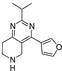
Example 150; 4-Furan-3-yl-2-isopropyl-5,6,7,8-tetrahydro-pyrido[4,3-d]pyrimidine.
