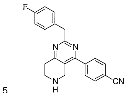
Example 16; 4-[2-(4-Fluoro-benzyl)-5,6,7,8-tetrahydro-pyrido[4,3-d]pyrimidin-4-yl]-benzonitrile.
