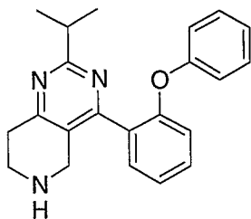
Example 33; 2-Isopropyl-4-(2-phenoxy-phenyl)-5,6,7,8-tetrahydro-pyrido[4,3-d]pyrimidine.
