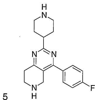
Example 131; 4-(4-Fluoro-phenyl)-2-piperidin-4-yl-5,6,7,8-tetrahydro-pyrido[4,3-d]pyrimidine.
