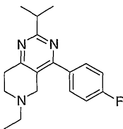
Example 159; 6-Ethyl-4-(4-fluoro-phenyl)-2-isopropyl-5,6,7,8-tetrahydro-pyrido[4,3-d]pyrimidine.
