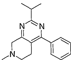
Example 85; 2-Isopropyl-7-methyl-4-phenyl-5,6,7,8-tetrahydro-pyrido[3,4-d]pyrimidine.
