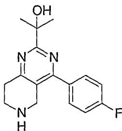
Example 127; 2-[4-(4-Fluoro-phenyl)-5,6,7,8-tetrahydro-pyrido[4,3-d]pyrimidin-2-yl]-propan-2-ol.
