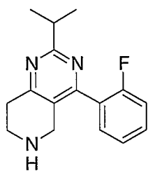
Example 26; 4-(2-Fluoro-phenyl)-2-isopropyl-5,6,7,8-tetrahydro-pyrido[4,3-d]pyrimidine.
