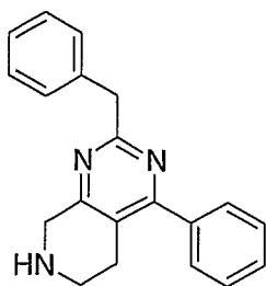
Example 78; 2-Benzyl-4-phenyl-5,6,7,8-tetrahydro-pyrido[3,4-d]pyrimidine.
