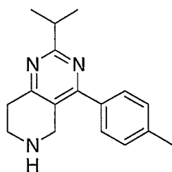
Example 28; 2-Isopropyl-4-p-tolyl-5,6,7,8-tetrahydro-pyrido[4,3-d]pyrimidine.
