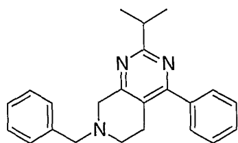
Example 74; 7-Benzyl-4-(4-fluoro-phenyl)-2-isopropyl-5,6,7,8-tetrahydro-pyrido[3,4-d]pyrimidine.
