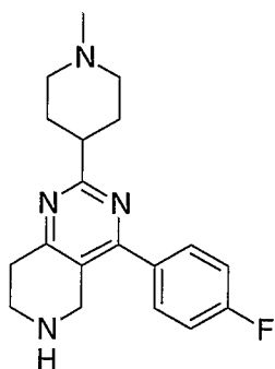
10 Example 132; 4-(4-Fluoro-phenyl)-2-(1-methyl-piperidin-4-yl)-5,6,7,8-tetrahydro-pyrido[4,3-d]pyrimidine.
