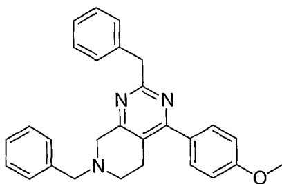
Example 73; 2,7-Dibenzyl-4-(4-methoxy-phenyl)-5,6,7,8-tetrahydro-pyrido[3,4-d]pyrimidine.
