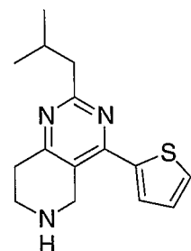
Example 35; 2-Isobutyl-4-thiophen-2-yl-5,6,7,8-tetrahydro-pyrido[4,3-d]pyrimidine.
