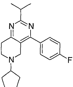
Example 162; 6-Cyclopentyl-4-(4-fluoro-phenyl)-2-isopropyl-5,6,7,8-tetrahydro-pyrido[4,3-d]pyrimidine.
