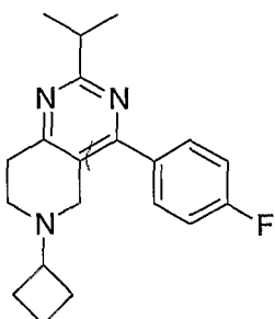
Example 161; 6-Cyclobutyl-4-(4-fluoro-phenyl)-2-isopropyl-5,6,7,8-tetrahydro-pyrido[4,3-d]pyrimidine.
