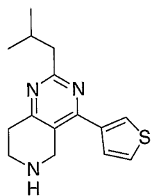
Example 34; 2-Isobutyl-4-thiophen-3-yl-5,6,7,8-tetrahydro-pyrido[4,3-d]pyrimidine.
