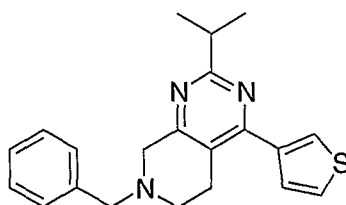
Example 87; 7-Benzyl-2-isopropyl-4-thiophen-3-yl-5,6,7,8-tetrahydro-pyrido[3,4-d]pyrimidine hydrochloride.
