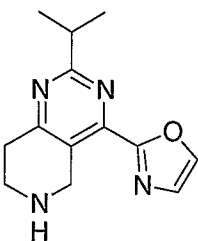
Example 152; 2-Isopropyl-4-oxazol-2-yl-5,6,7,8-tetrahydro-pyrido[4,3-d]pyrimidine.
