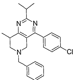
Example 97; 6-Benzyl-4-(4-chloro-phenyl)-2-isopropyl-8-methyl-5,6,7,8-tetrahydro-pyrido[4,3-d]pyrimidine.
