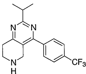
Example 32; 2-Isopropyl-4-(4-trifluoromethyl-phenyl)-5,6,7,8-tetrahydro-pyrido[4,3-d]pyrimidine.
