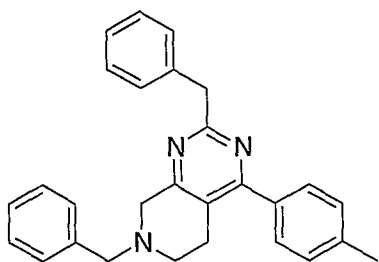
Example 71; 2,7-Dibenzyl-4-p-tolyl-5,6,7,8-tetrahydro-pyrido[3,4-d]pyrimidine.
