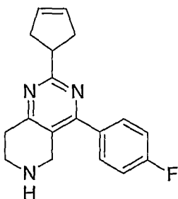
Example 129; 2-Cyclopent-3-enyl-4-(4-fluoro-phenyl)-5,6,7,8-tetrahydro-pyrido[4,3-d]pyrimidine.
