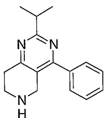
10 Example 31; 2-Isopropyl-4-phenyl-5,6,7,8-tetrahydro-pyrido[4,3-d]pyrimidine.
