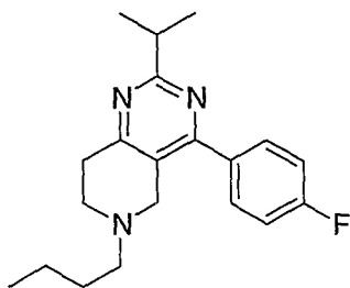
Example 163; 6-Butyl-4-(4-fluoro-phenyl)-2-isopropyl-5,6,7,8-tetrahydro-pyrido[4,3-d]pyrimidine.
