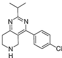
Example 29; 4-(4-Chloro-phenyl)-2-isopropyl-5,6,7,8-tetrahydro-pyrido[4,3-d]pyrimidine.
