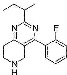
10 Example 42; 2-sec-Butyl-4-(2-fluoro-phenyl)-5,6,7,8-tetrahydro-pyrido[4,3-d]pyrimidine hydrochloride.
