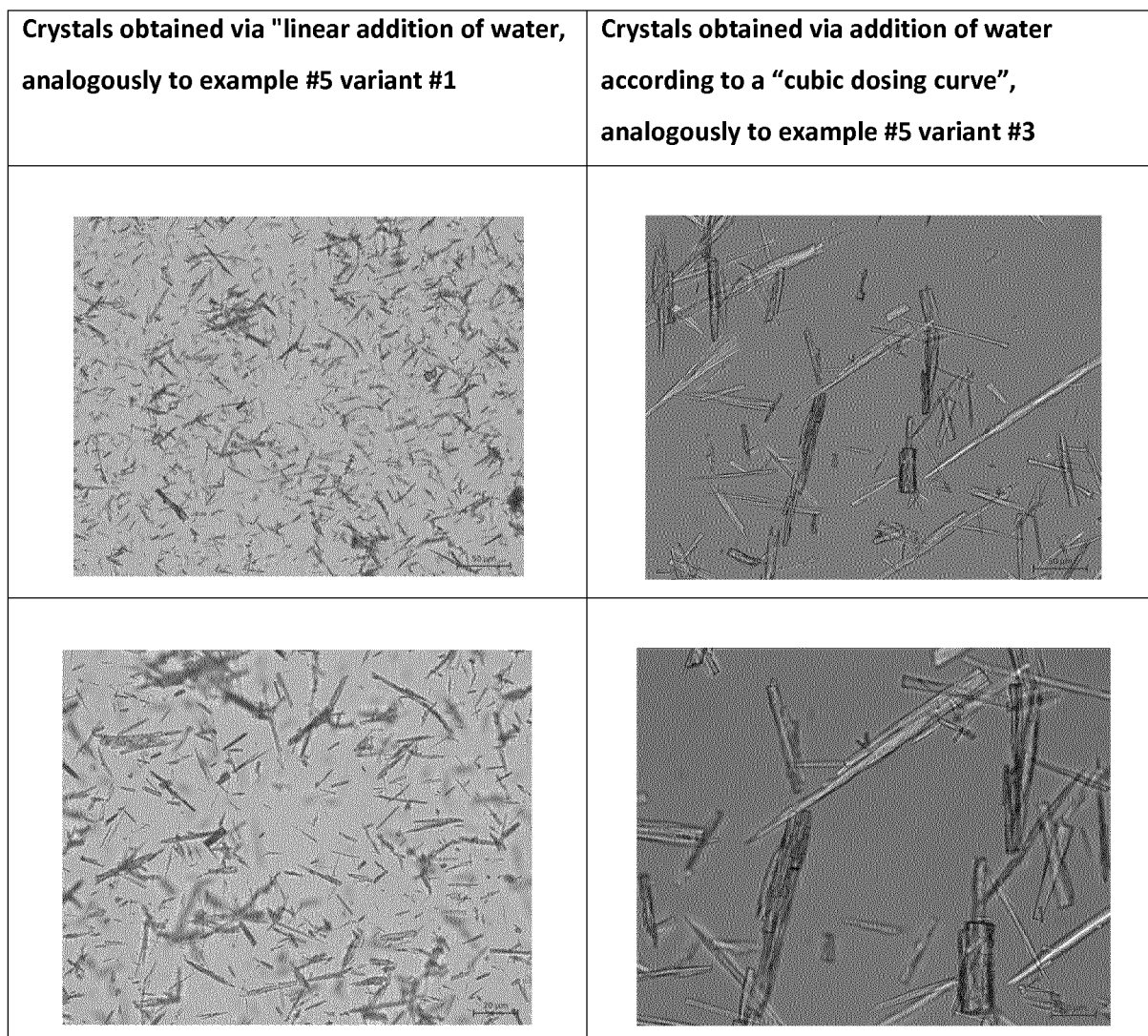
Figure 2: Microscopic images of crystalline particles of (I) obtained via recrystallization analogous to the recrystallization protocol described in example #5 variant #1 compared to crystalline particles of (I) obtained analogous to the recrystallization described in example #5, variant #3
