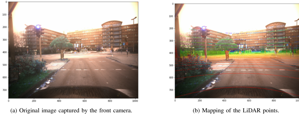
Fig. 5. LiDAR points mapping using vehicle coordinate system.
