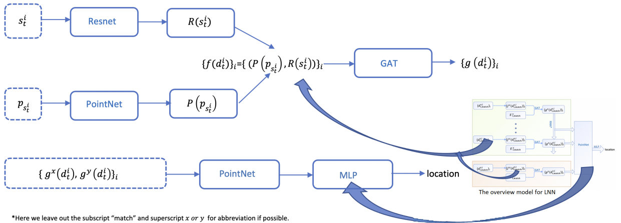
Fig. 13. LNN architecture.
