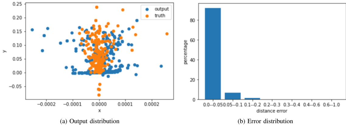
Fig. 16. Ground truth and model output comparison in the real dataset.
