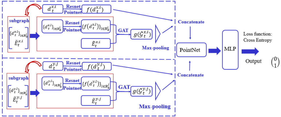
Fig. 10. Matching model based on GAT for landmark segmentations.
