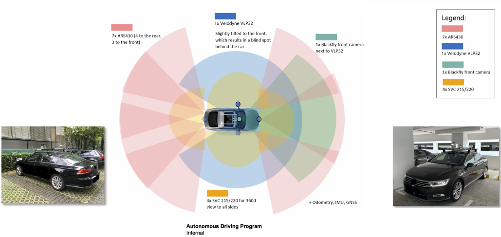
Fig. 3. Sensors equipped in the vehicle.
