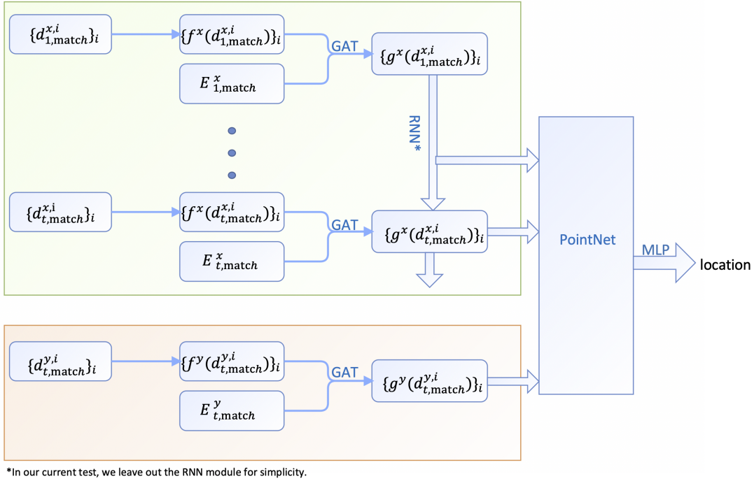
Fig. 12. The overview model for LNN.
