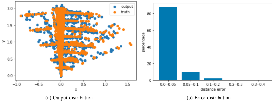
Fig. 15. Ground truth and model output comparison in CARLA dataset 1 with L = 2 .
