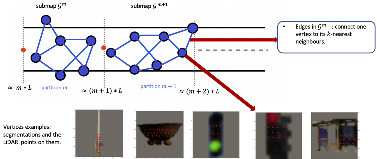
Fig. 7. The graph topological landmark map constructed in each road partition and examples of vertices in the map graph.
