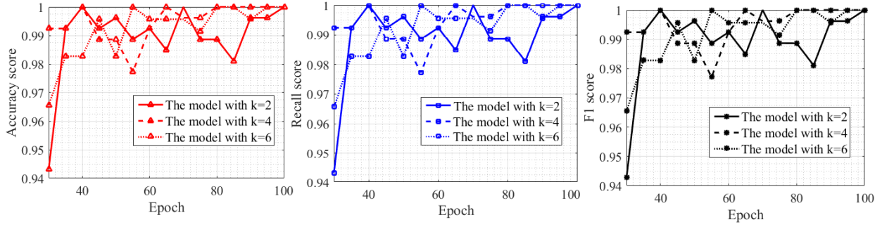
Fig. 11. Experiment results for the matched pairs of landmark segmentations including traffic lights, traffic signs and lamp posts.
