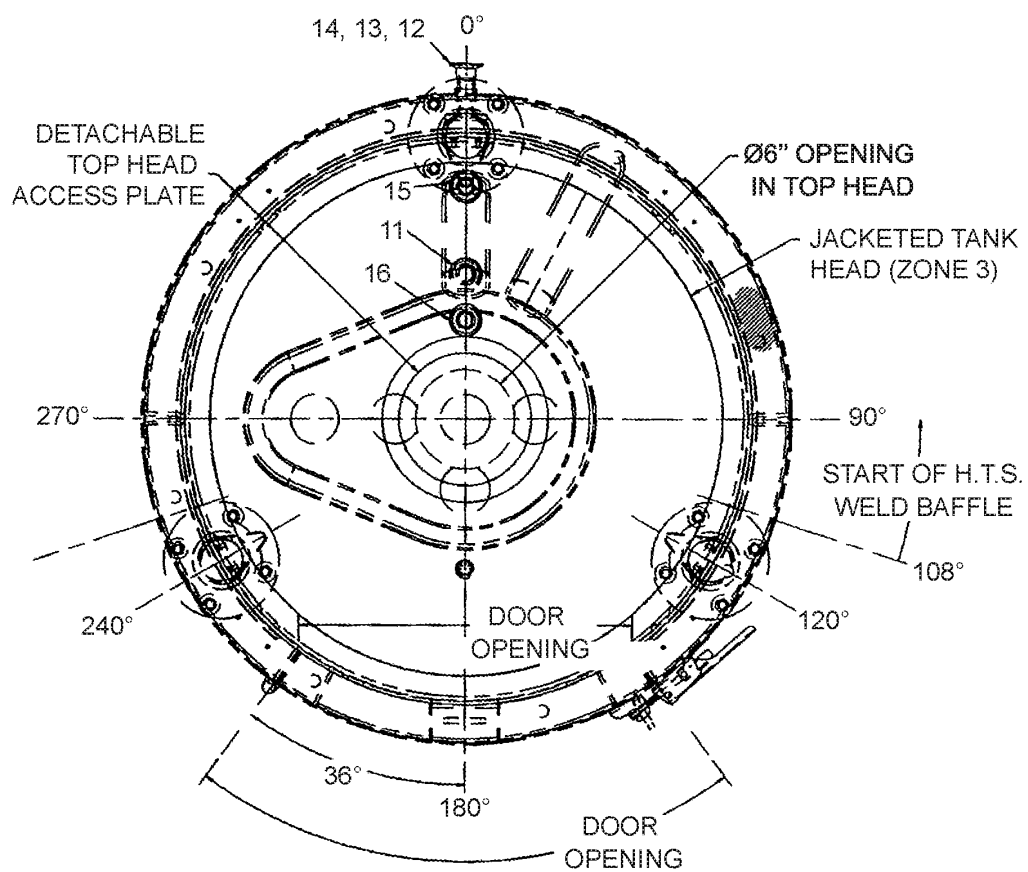
PLAN VIEW
