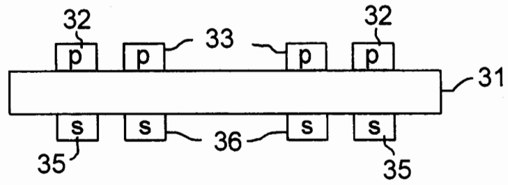
FIG. 3 (prior art)
