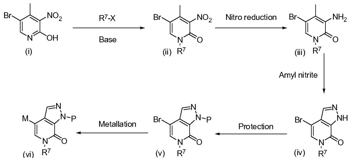
Scheme VIII
