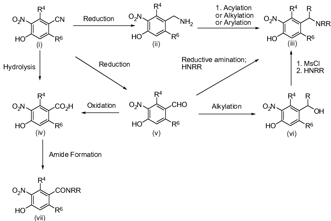
Scheme V
