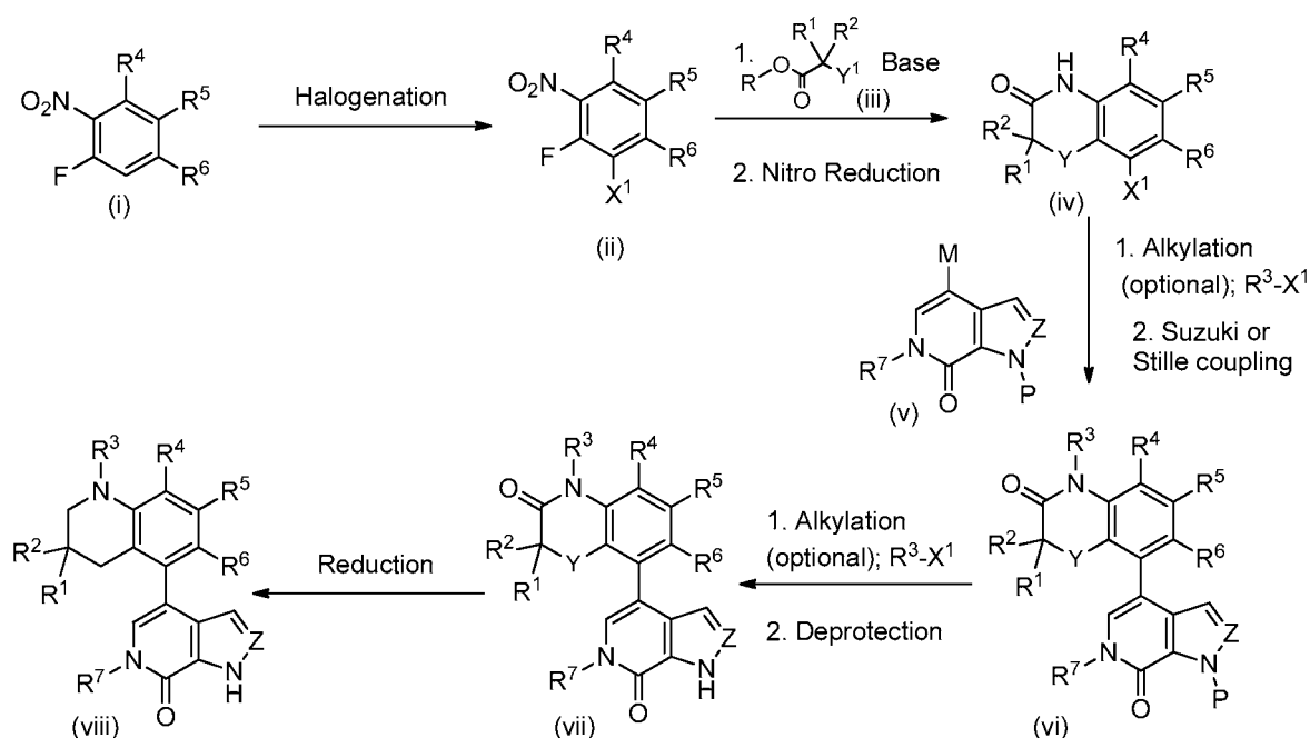
Scheme III
