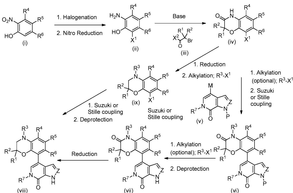
Scheme II
