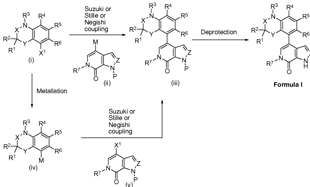
Scheme I
