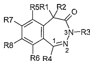
substituted 3,5-dihydro-4H-2,3-benzodiazepin-4-ones
