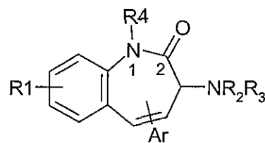
substituted 3-amino-2,3-dihydro-1H-1-benzazepin-2-ones
