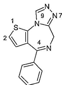
4-phenyl-6H-thieno[3,2-f][1,2,4]triazolo[4,3-a][1,4]diazepine
