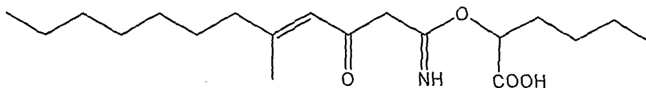
(IX)
