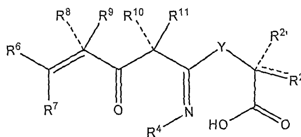
(IIIa)
