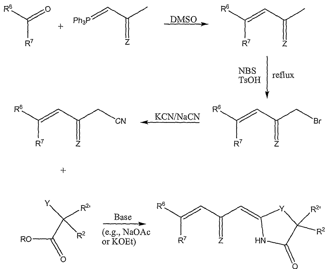
Scheme A
