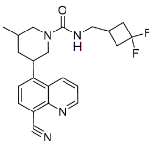
Compound 110
