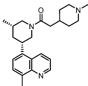
Compound 82
