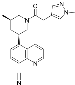
Compound 107
