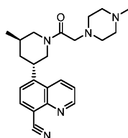
Compound 96
