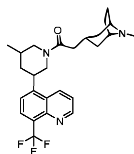
Compound 18
