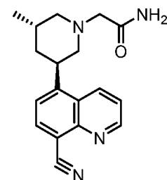
Compound 66
