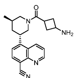
Compound 99
