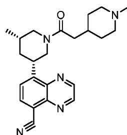
Compound 102
