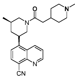
Compound 1
