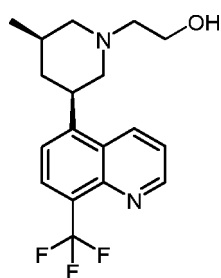
Compound 7
