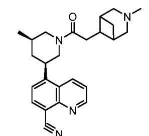
Compound 93
