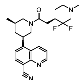
Compound 91
