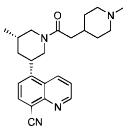
Compound 56
