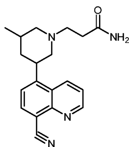
Compound 49
