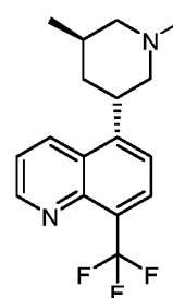
Compound 6
