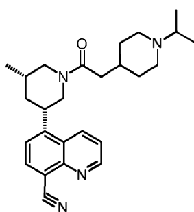
Compound 47
