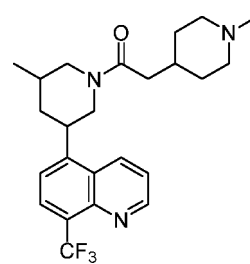
Compound 3
