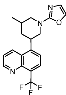
Compound 59
