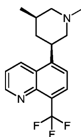
Compound 5
