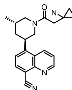
Compound 63
