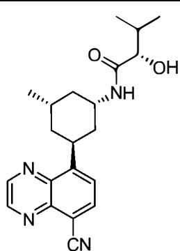
Compound 128
