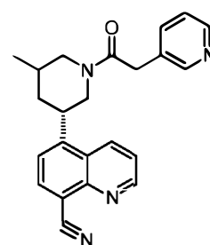
Compound 21
