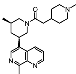
Compound 95
