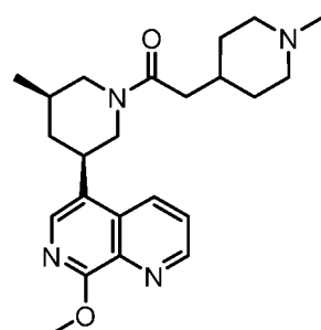
Compound 89
