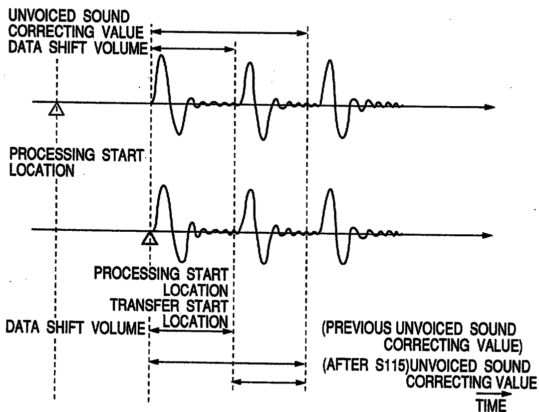
DATA SHIFT VOLUME 1k < UNVOICED SOUND CORRECTING VALUE 1o (S115)
