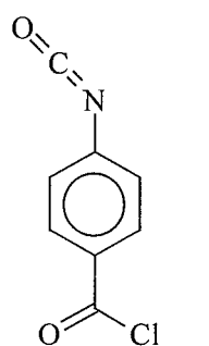
4-isocyanato- benzoylchloride
