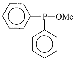
methoxydiphenyl- phosphineoxide
