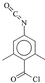
4-isocyanato-3,5-dimethyl benzoylchloride
