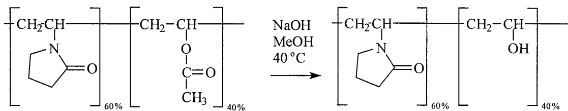
poly(NVP-co-VAc) 60/40
