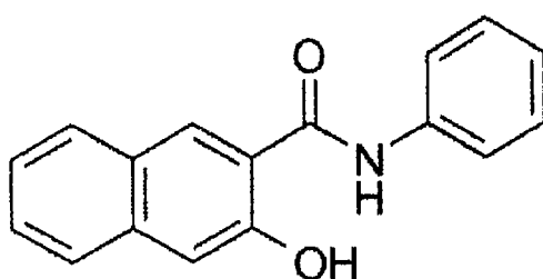
Naphtol AS
