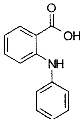
N-phenylanthranilic acid
