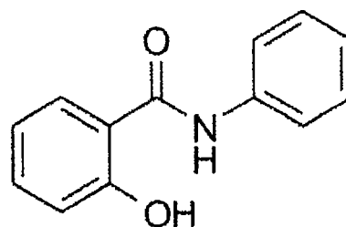
salicylanilide
