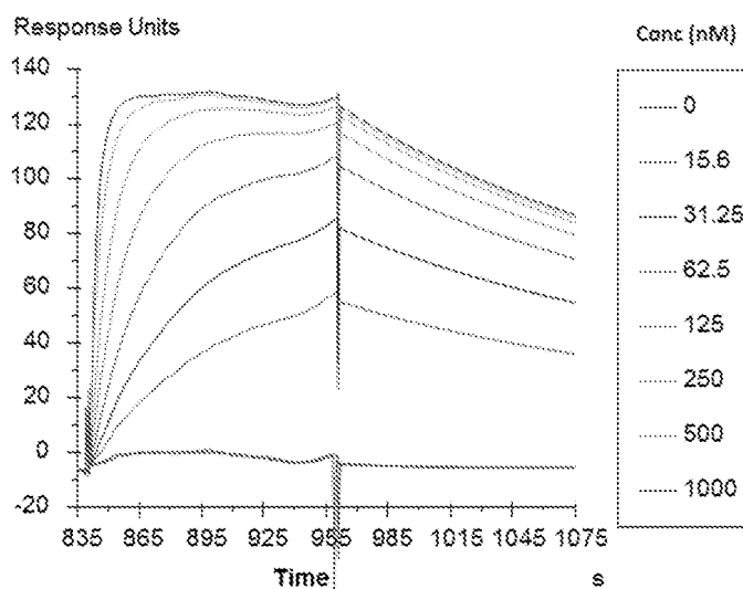
B: Sensorgram showing the association and dissociation phases of CD200R binding to captured K130Y
