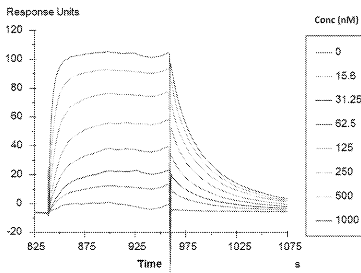
A: Sensorgram showing the association and dissociation phases of CD200R binding to captured WT CD200
