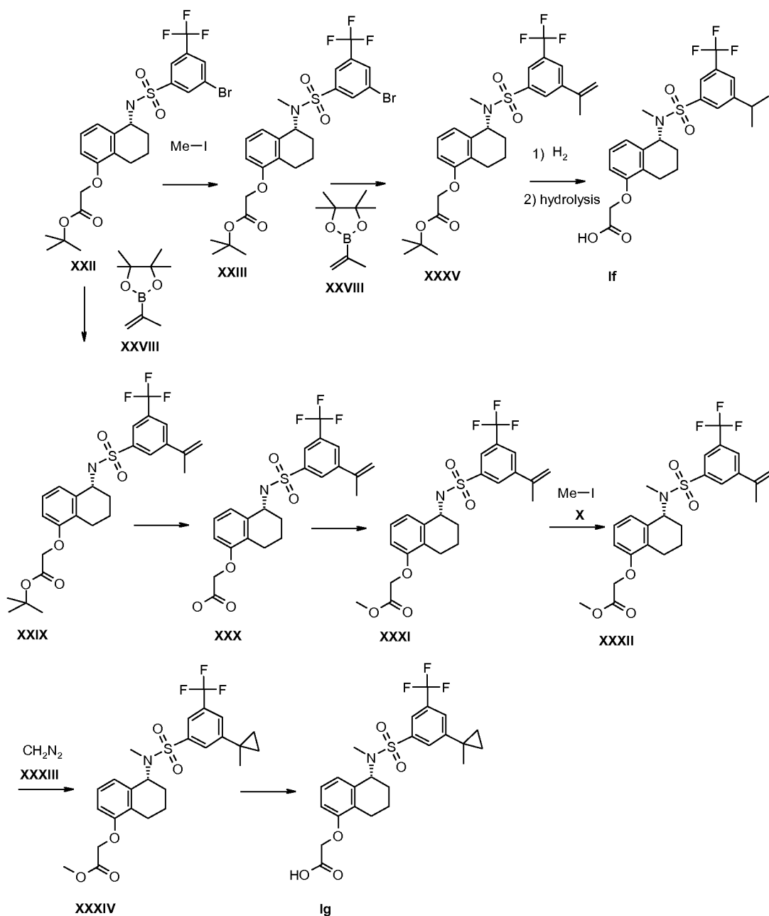
Scheme 6
