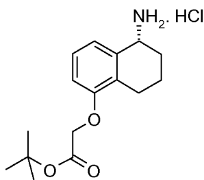
((S)-5-hydroxy-5,6,7,8-tetrahydro-naphthalen-1-yloxy)-acetic acid tert -butyl ester (XI)
