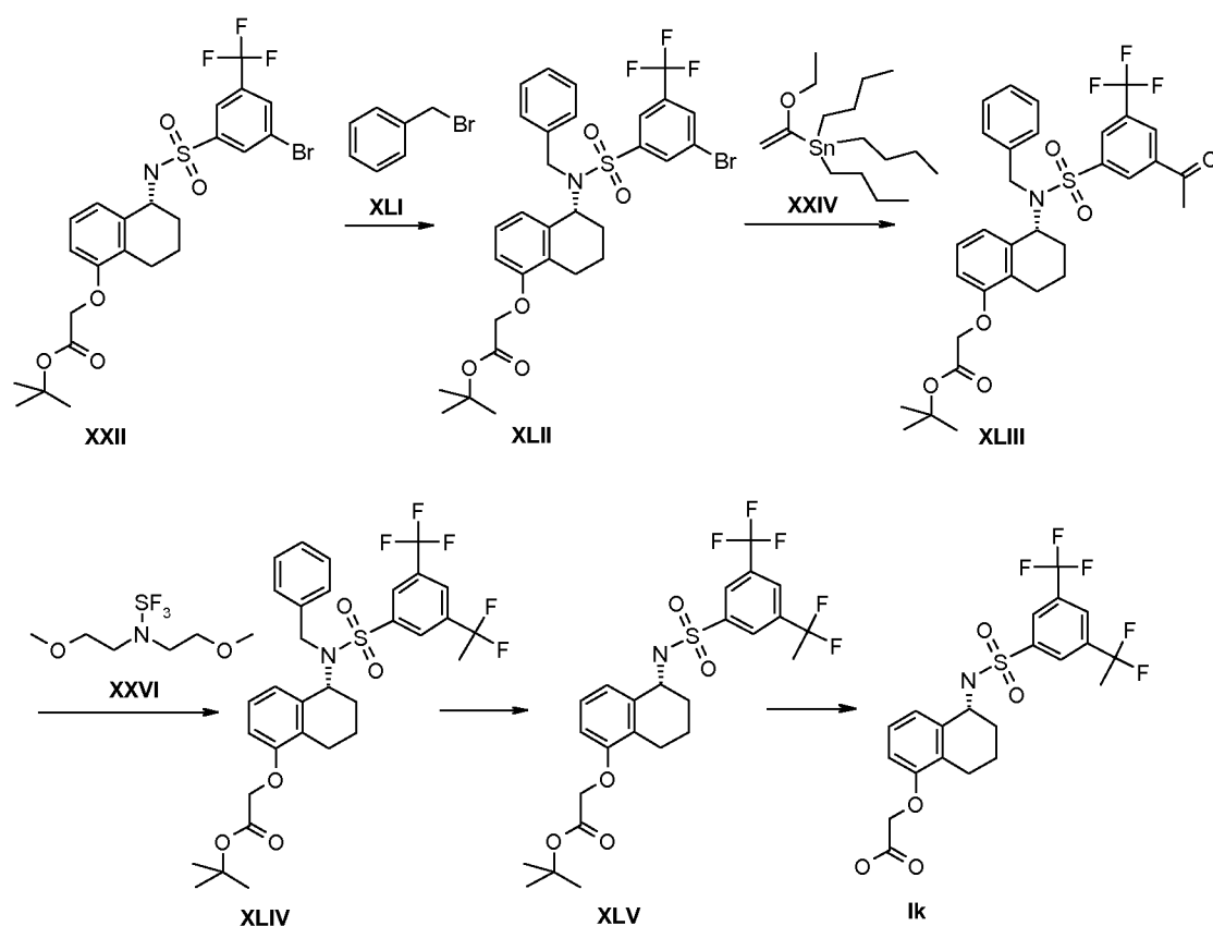
Scheme 10
