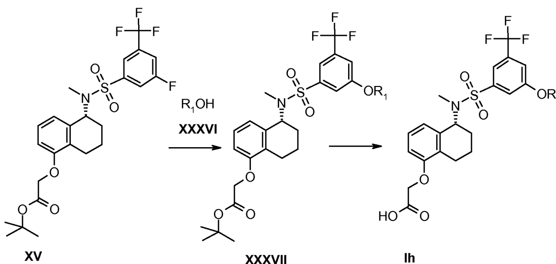
Scheme 7
