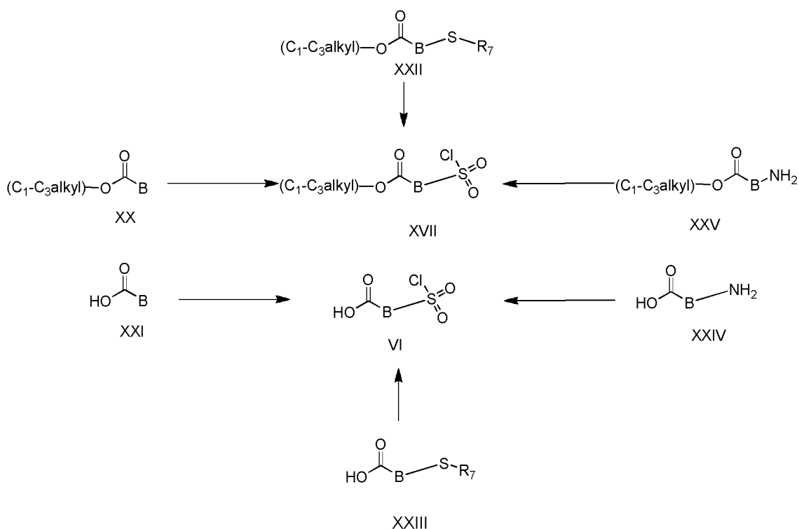
Scheme 7
