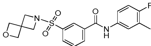
Compound 135
