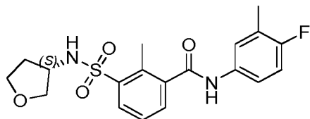
Compound 126
