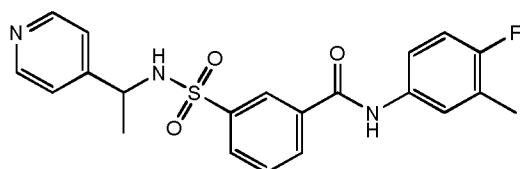
Compound 161
