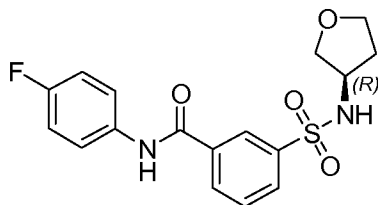
Compound 8
