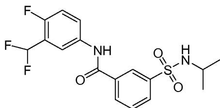
Compound 96
