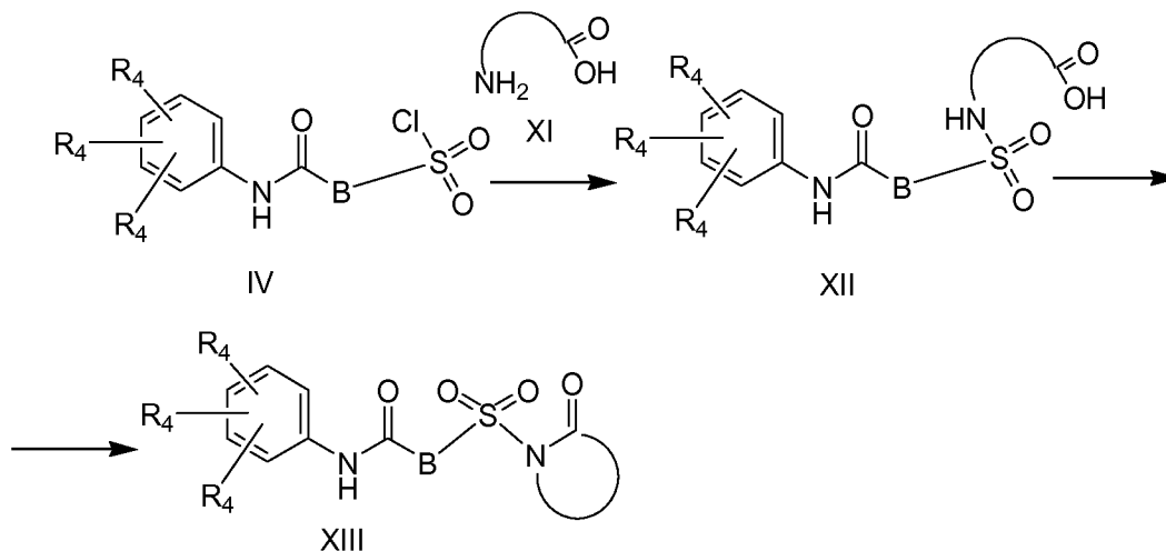
Scheme 4
