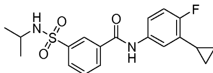
Compound 84
