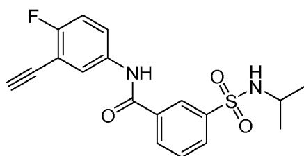
Compound 91
