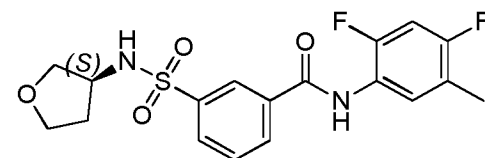
Compound 106
