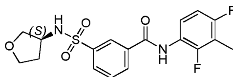
Compound 104
