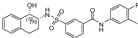
Compound 137
