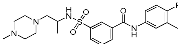
Compound 116
