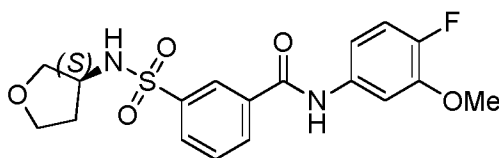
Compound 103
