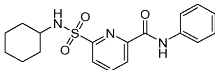
Compound 65
