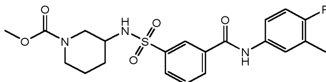
Compound 159
