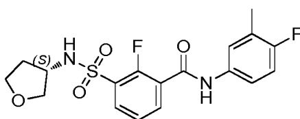
Compound 112
