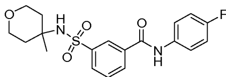
Compound 83
