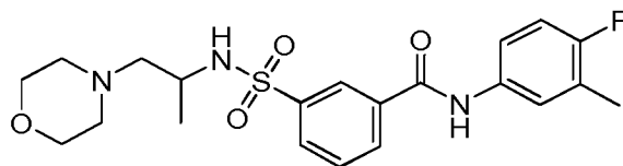
Compound 117
