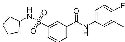
Compound 11
