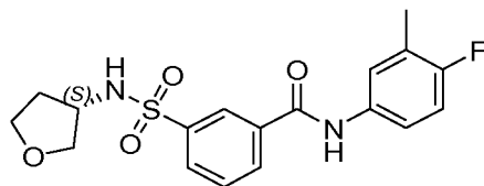
Compound 72
