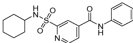
Compound 66
