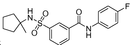
20 Compound 76
