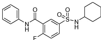
Compound 19
