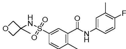
Compound 122
