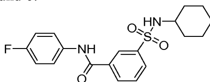
Compound 6
