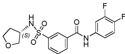
Compound 90
