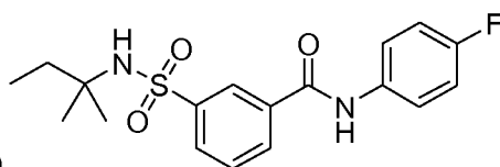
Compound 79
