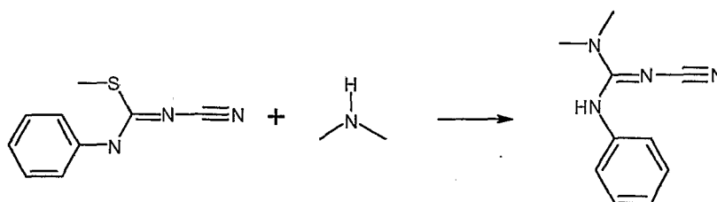
Scheme 13
