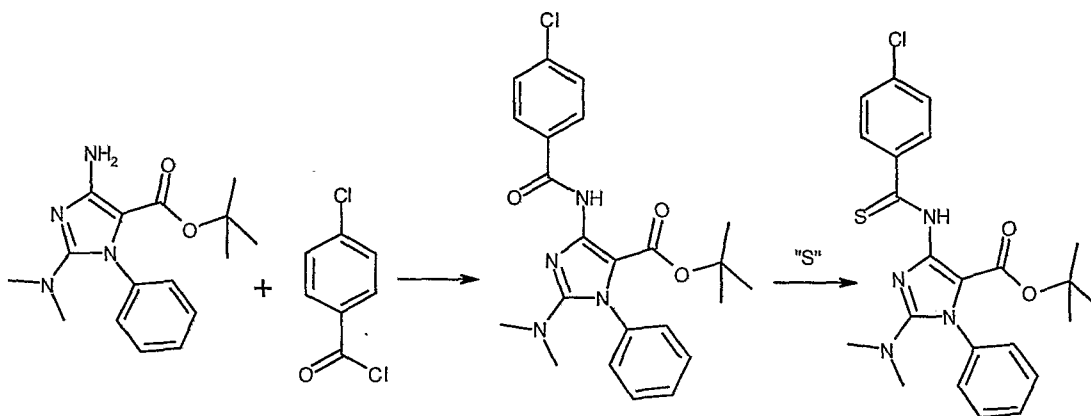
Scheme 8
