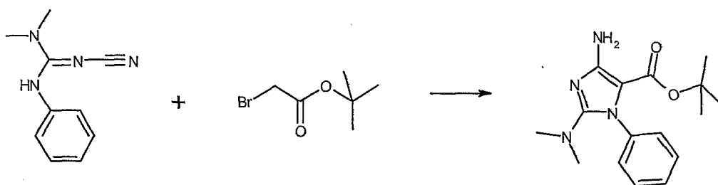
Scheme 10
