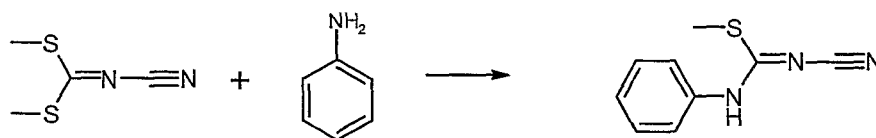
Scheme 12
