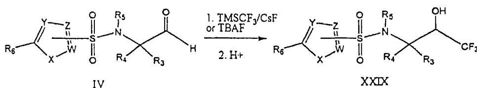
Scheme 9
