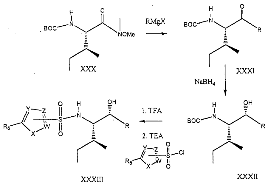
Scheme 10
