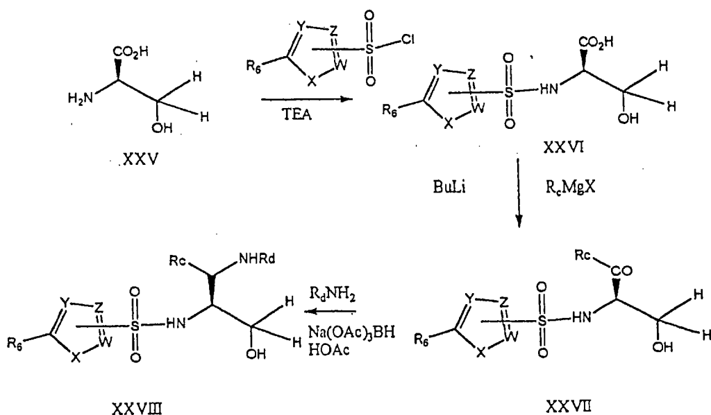
Scheme 8
