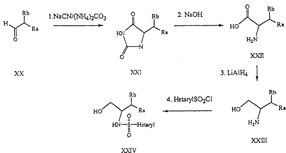
Scheme 7
