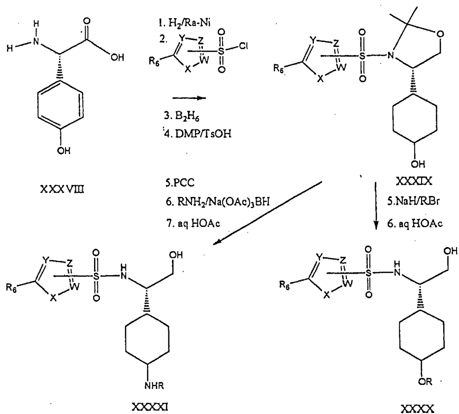
Scheme 12
