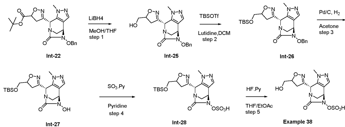
Scheme 5
