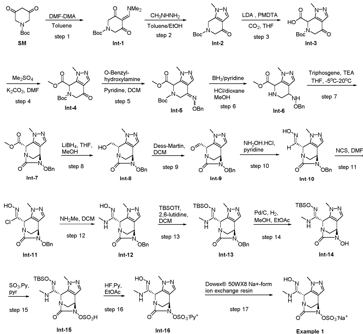
Scheme 1
