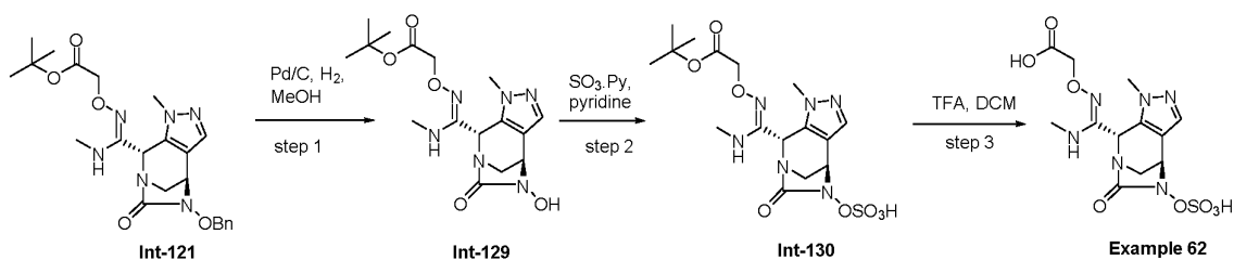
Scheme 24
