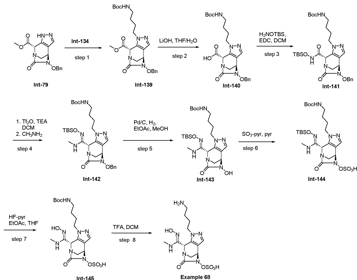
Scheme 30
