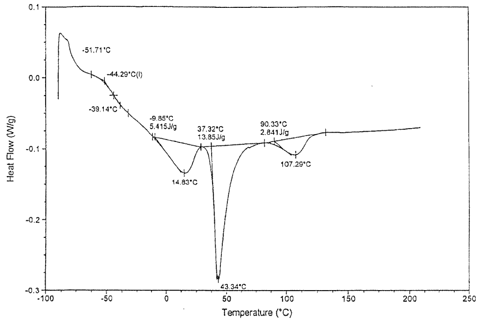
Fig. 3 DSC for Example 2
