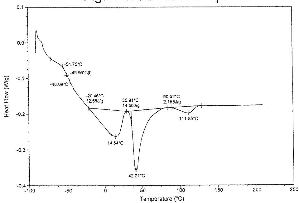
Fig. 2 DSC for Example 1
