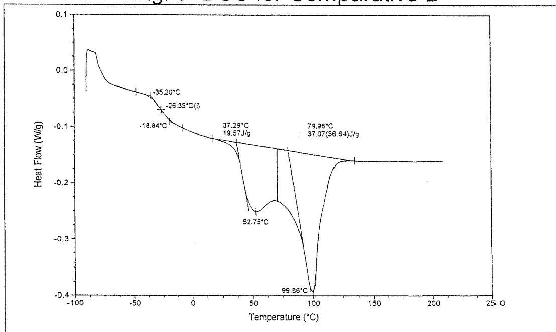
Fig. 6 DSC for Comparative B
