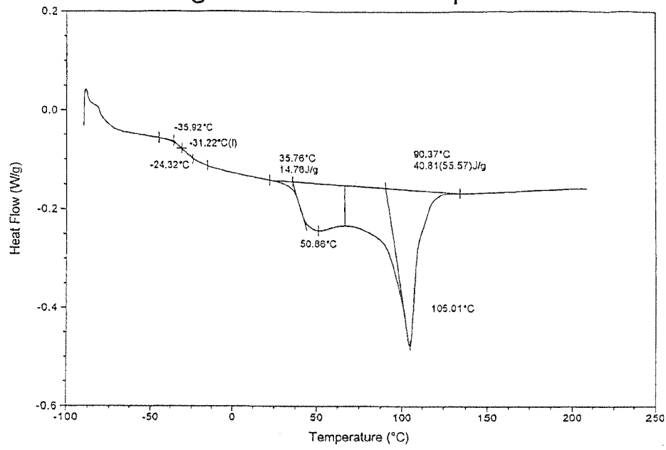
Fig. 5 DSC for Comparative A
