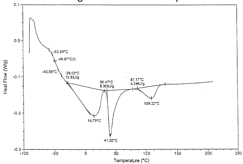
Fig. 4 DSC for Example 3
