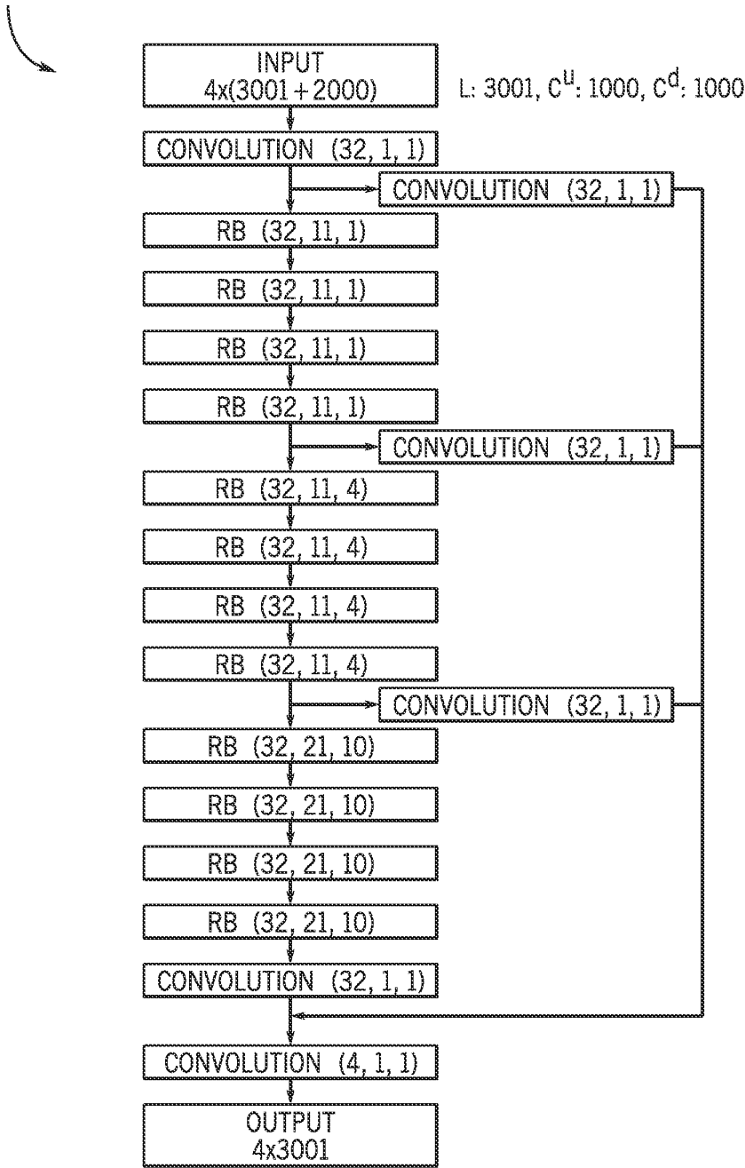
EXAMPLE ARCHITECTURE 1100 OF CHROMATIN MODEL 802
