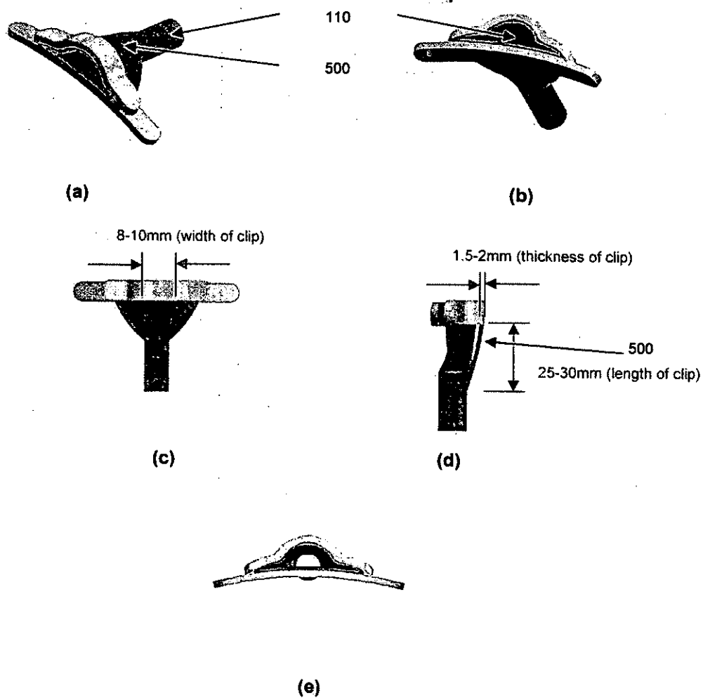
Figure 6: Nozzle design with clip
