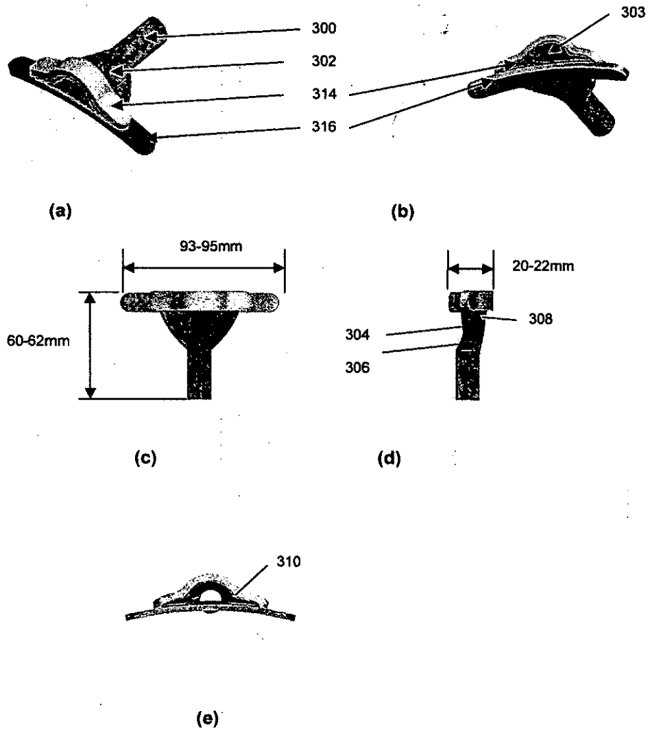
Figure 4: Nozzle design without clip
