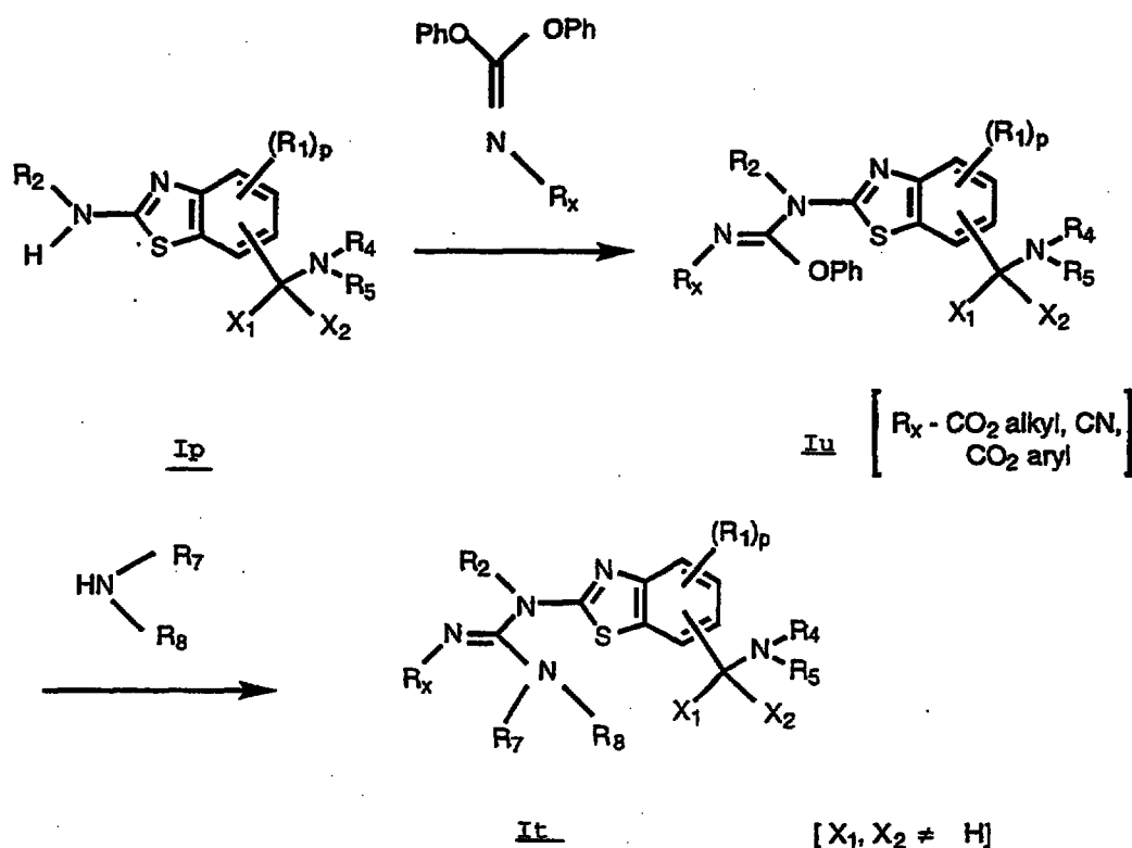
Scheme IX
