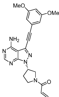
TAS-120;
