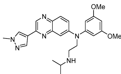
Erdafitinib;
