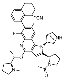
Compound 6;
