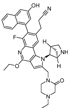
(Compound 7).
