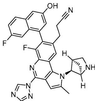
Compound 5;
