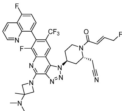
Compound 3;
