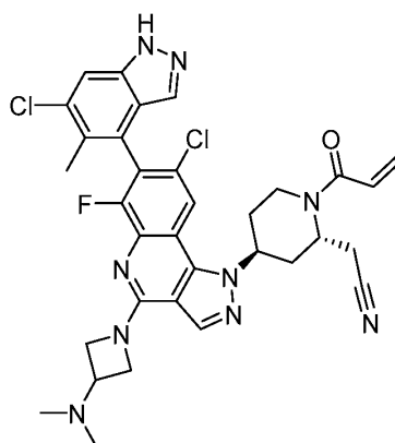
Compound 4;
