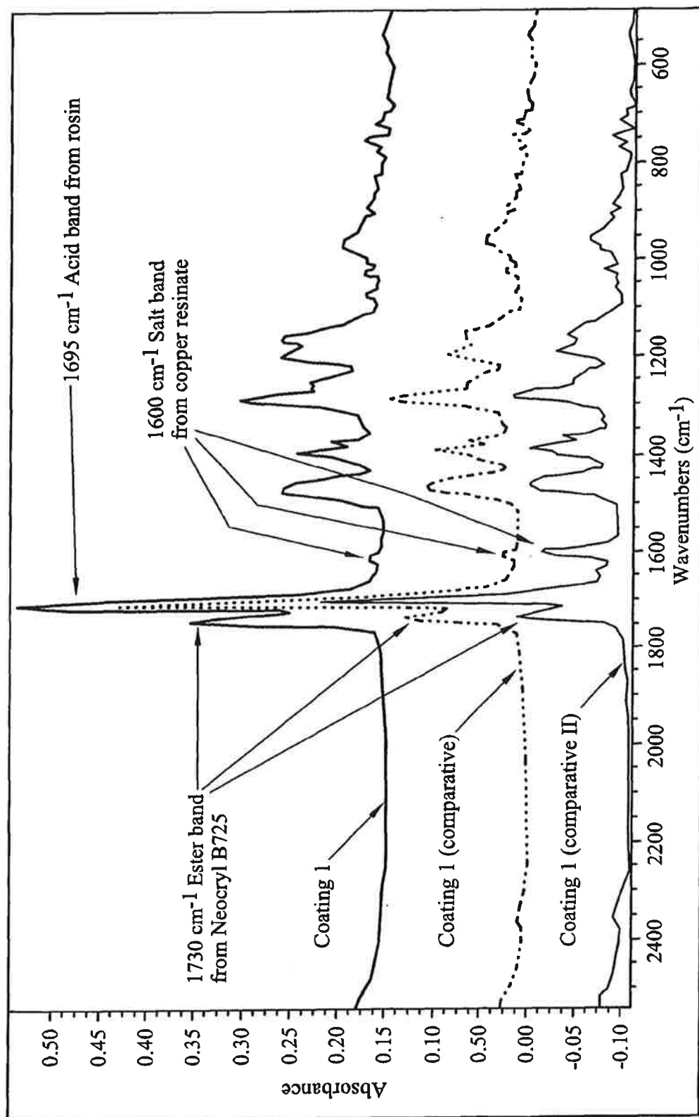
IR spectra of binder part of coatings based on Neocryl B725 & rosin
