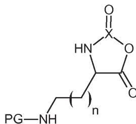
Formula II
