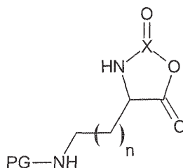
Formula II
