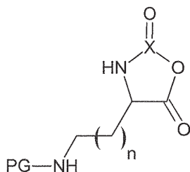
Formula II
