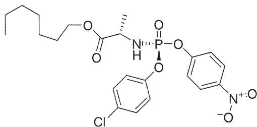
Compound 19
