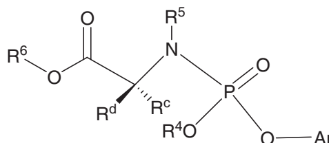
Formula VIII
