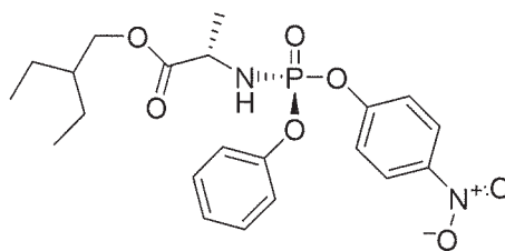
Compound 15
