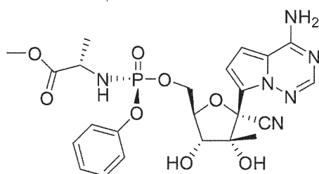
Compound 22
