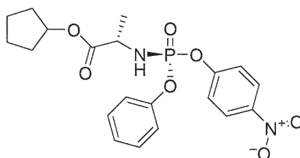
Compound 16
