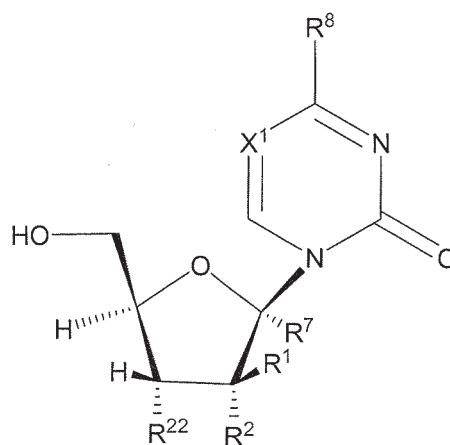
Formula XIV
