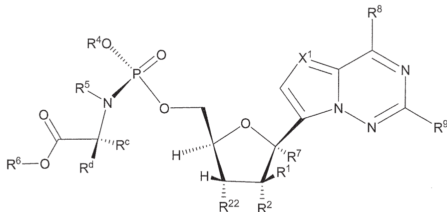
Formula VIb
