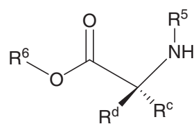
Formula IX
