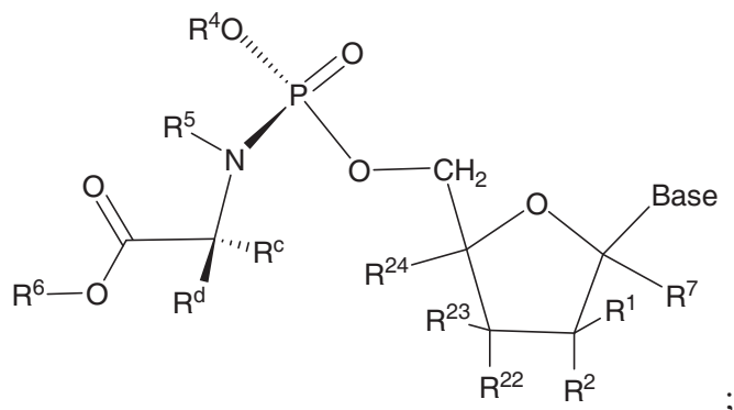
Formula Ib
