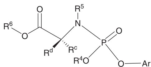
Formula VIII
