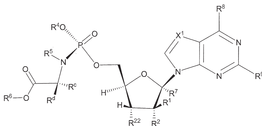
Formula XIb
