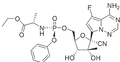
Compound 30
