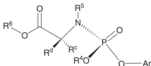
Formula IIIb
