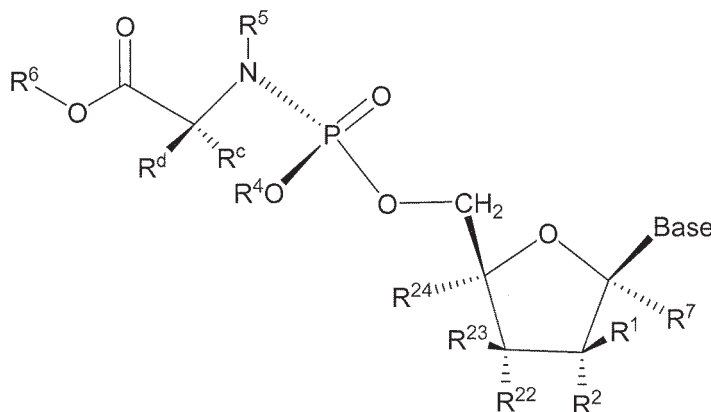
Formula IVa
