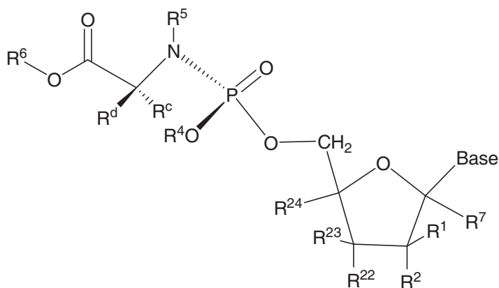
Formula Ia
