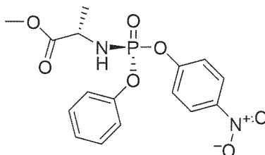
Compound 10
