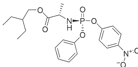
Compound 13
