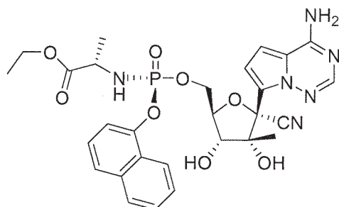
Compound 29
