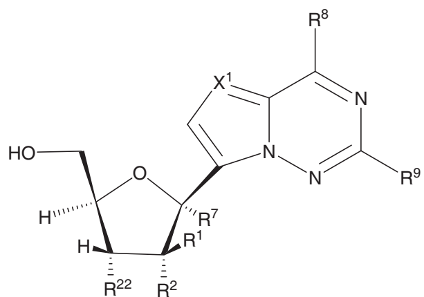
Formula VII
