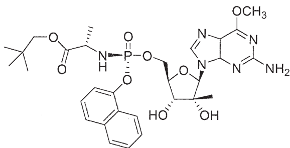
Compound 36
