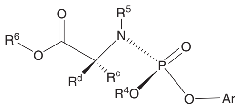
Formula IIIb
