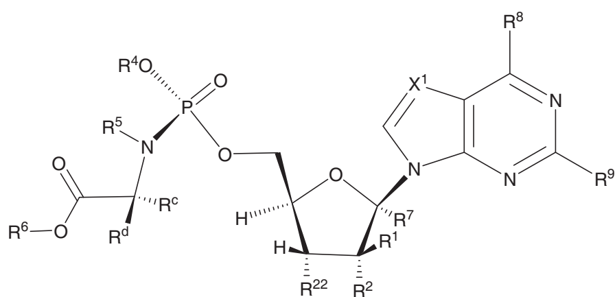
Formula XIb
