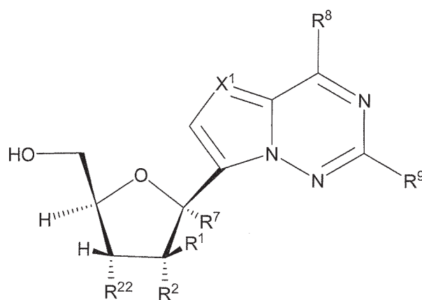
Formula VII
