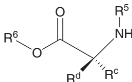
Formula IX
