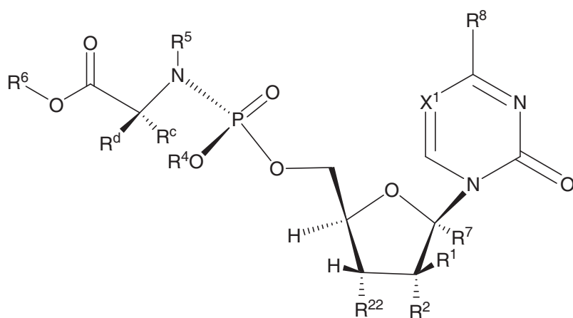
Formula XIIIa
