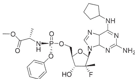
Compound 38
