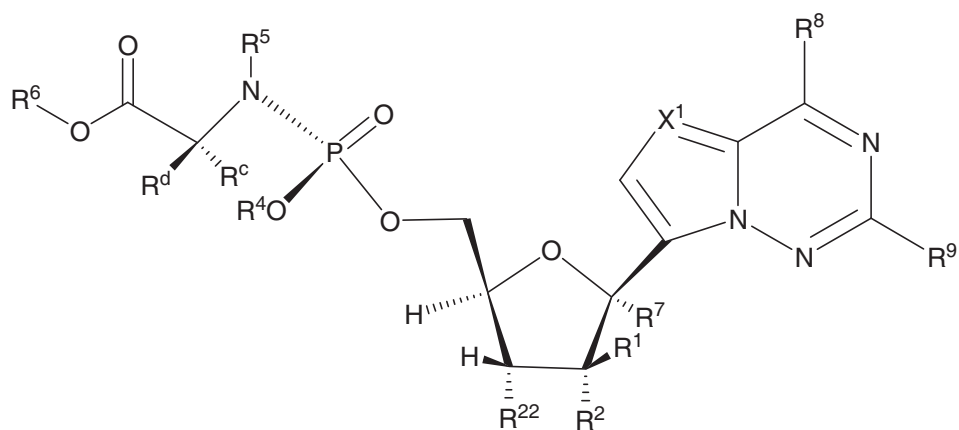
Formula VIa
