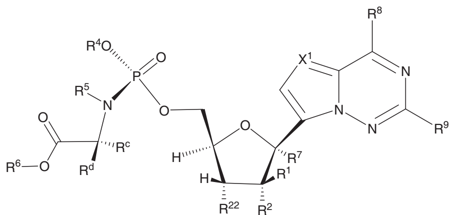
Formula VIb
