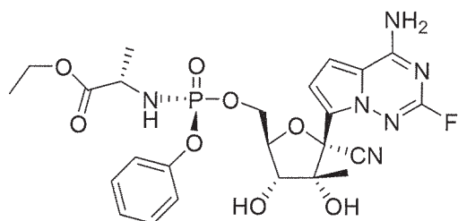
Compound 31
