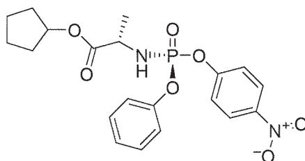
Compound 17
