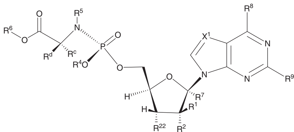
Formula XIa
