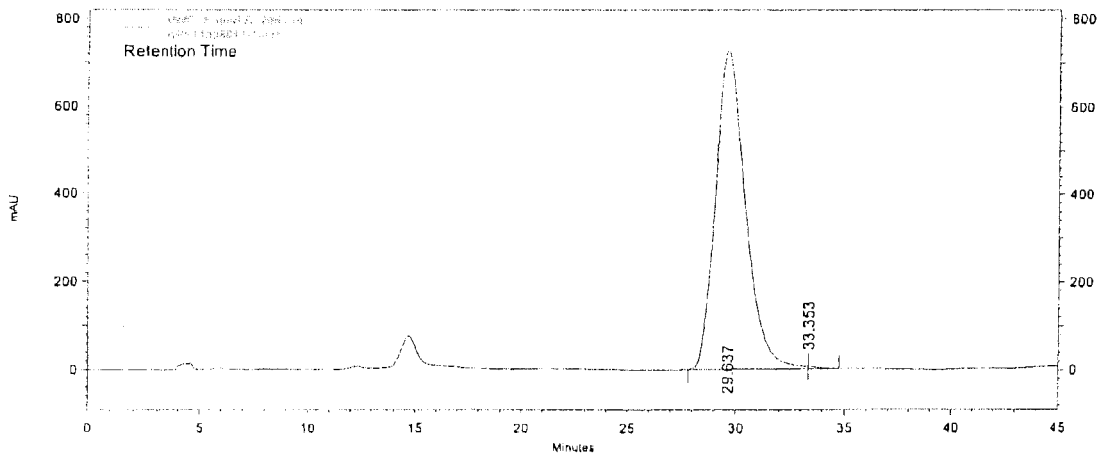
CHIRAL HPLC OF ISOMER 1
