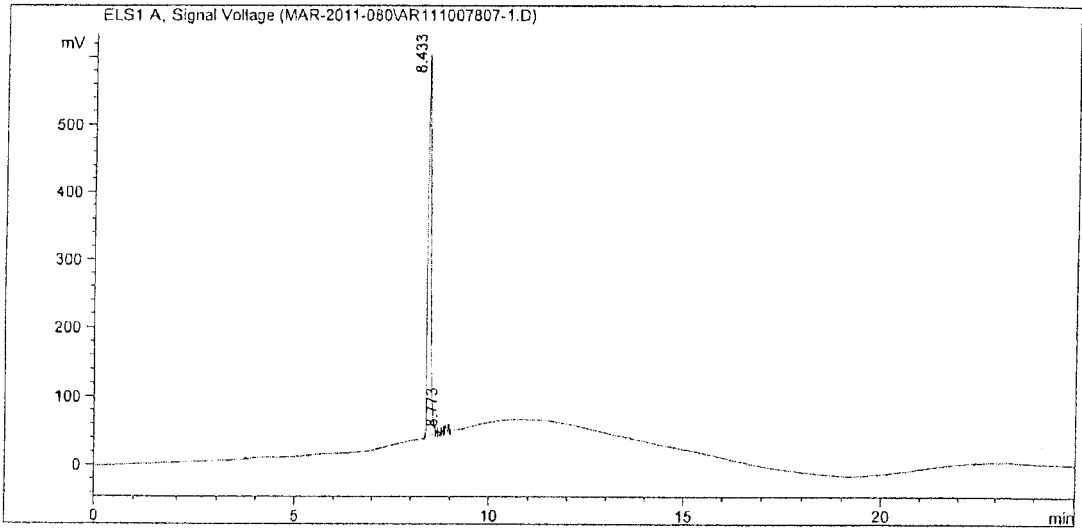
HPLC OF ISOMER 1
