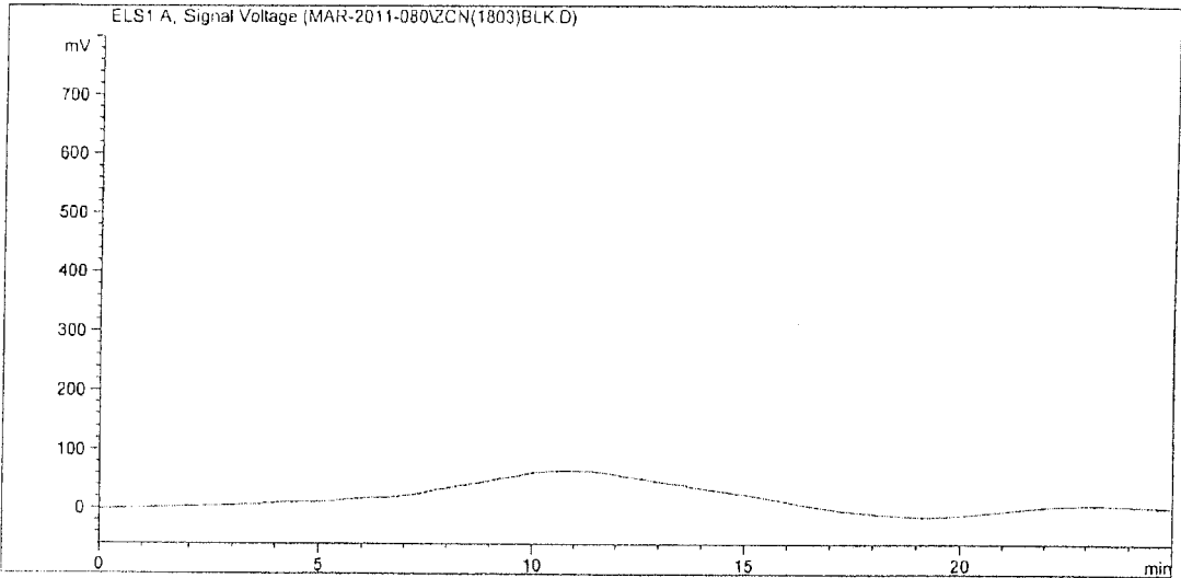
HPLC BLANK ISOMER 1
