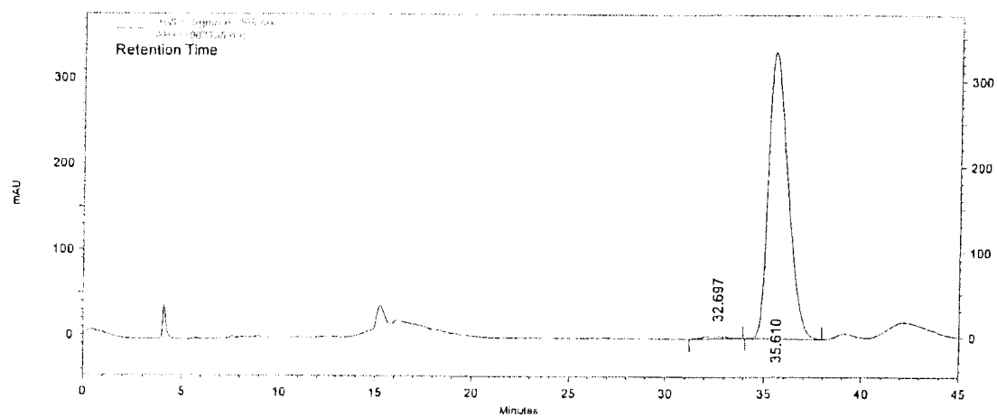
CHIRAL HPLC ISOMER 2
