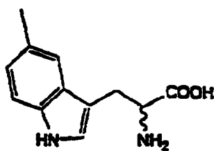
DL-5-Mc-Trp
