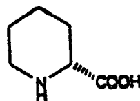
D-Pipecolic acid
