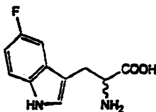
DL-5-F-Trp
