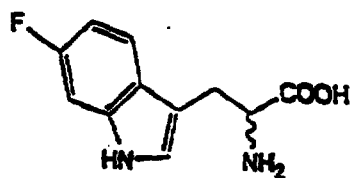
DL-6-F-Trp
