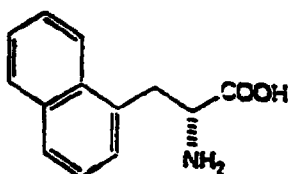
D-1-Nal
