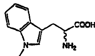
DL-1-Mc-Trp
