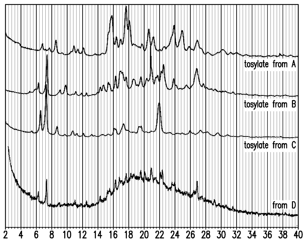
Overlay Plot of Forms A, B, C, and D of a Tosylate Salt of Compound 1
