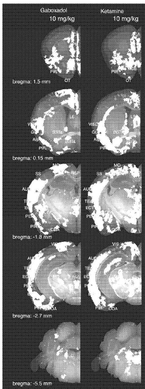
Figure 26: Gaboxadol and Ketamine side-by-side pharmacomap comparison
