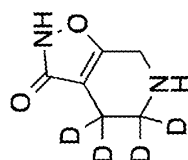
4,5,6,7-tetrahydroisoxazolo[5,4-c]pyridin-3(2H)-one-4,4,5,5- d_4
