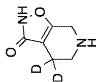
4,5,6,7-tetrahydroisoxazolo[5,4-c]pyridin-3(2H)-one-4,4- d_2
