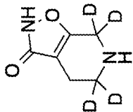
4,5,6,7-tetrahydroisoxazolo[5,4-c]pyridin-3(2H)-one-5,5,7,7- d_4
