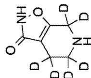
4,5,6,7-tetrahydroisoxazolo[5,4-c]pyridin-3(2H)-one-4,4,5,5,7,7- d_6
