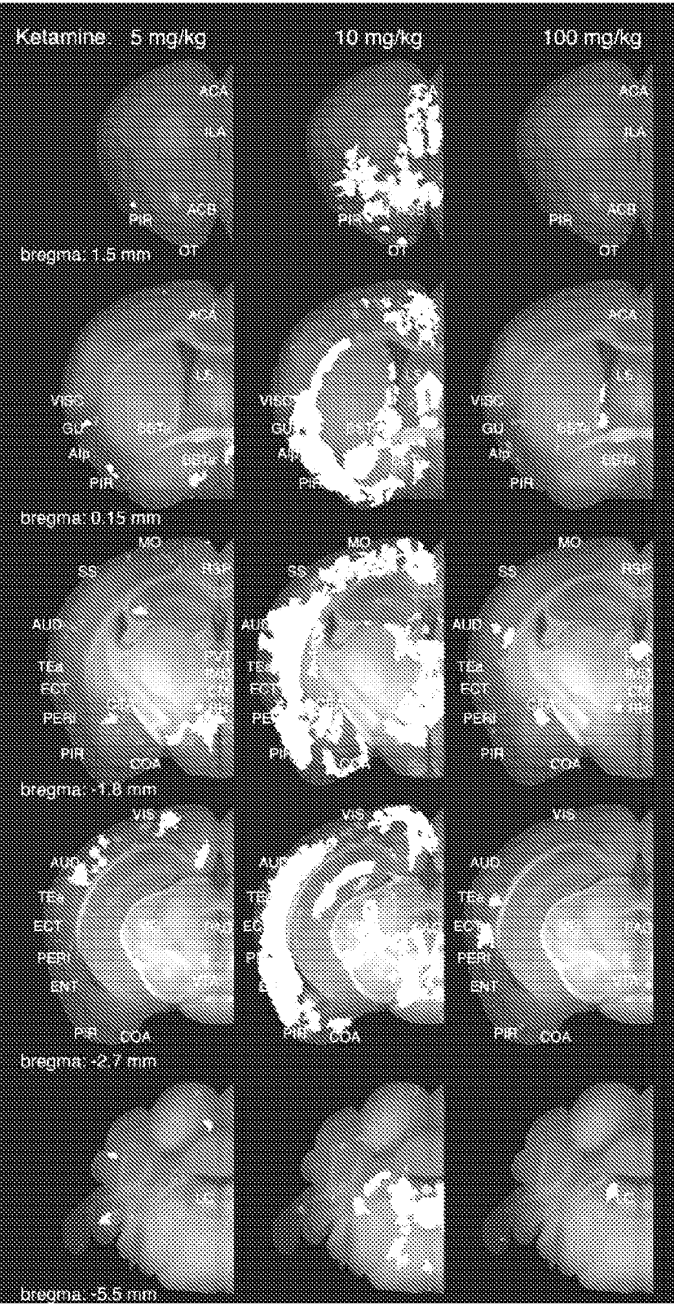
Figure 25: Ketamine dose-curve pharmacomaps.
