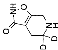
4,5,6,7-tetrahydroisoxazolo[5,4-c]pyridin-3(2H)-one-5,5- d_2
