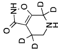
4,5,6,7-tetrahydroisoxazolo[5,4-c]pyridin-3(2H)-one-4,4,7,7- d_4
