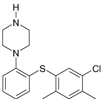
1-[2-(5-chloro-2,4-dimethyl-phenylsulfanyl)phenyl]piperazine
