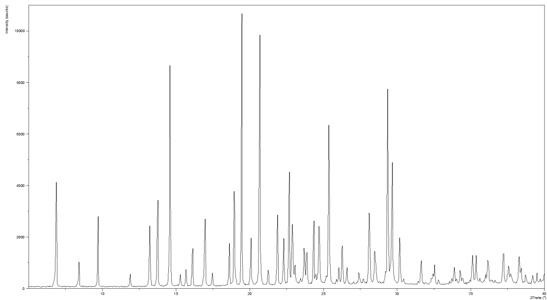
XRPD of 1-[2-(2,4-dimethylphenylsulfanyl)phenyl]piperazine, HBr, \beta -form
